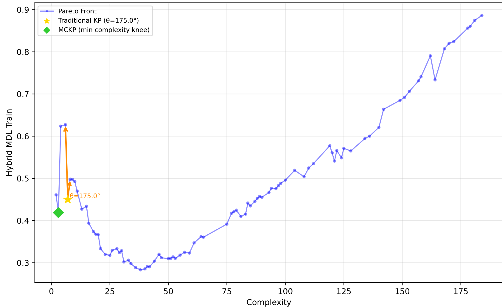
561_cpu - Run 16 - MVP - Hybrid MDL Train \lambda_1=0.50, \lambda_2=0.20, \lambda_3=0.00 | Difficulty: 0.94 | Method: hmr
