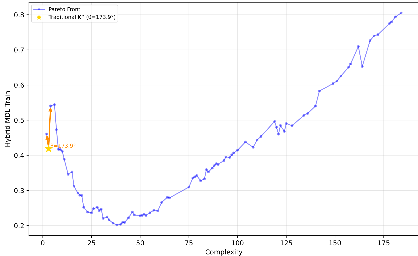
561_cpu - Run 16 - MVP - Hybrid MDL Train \lambda_1=0.70, \lambda_2=0.00, \lambda_3=0.10 | Difficulty: 0.94 | Method: hmr
