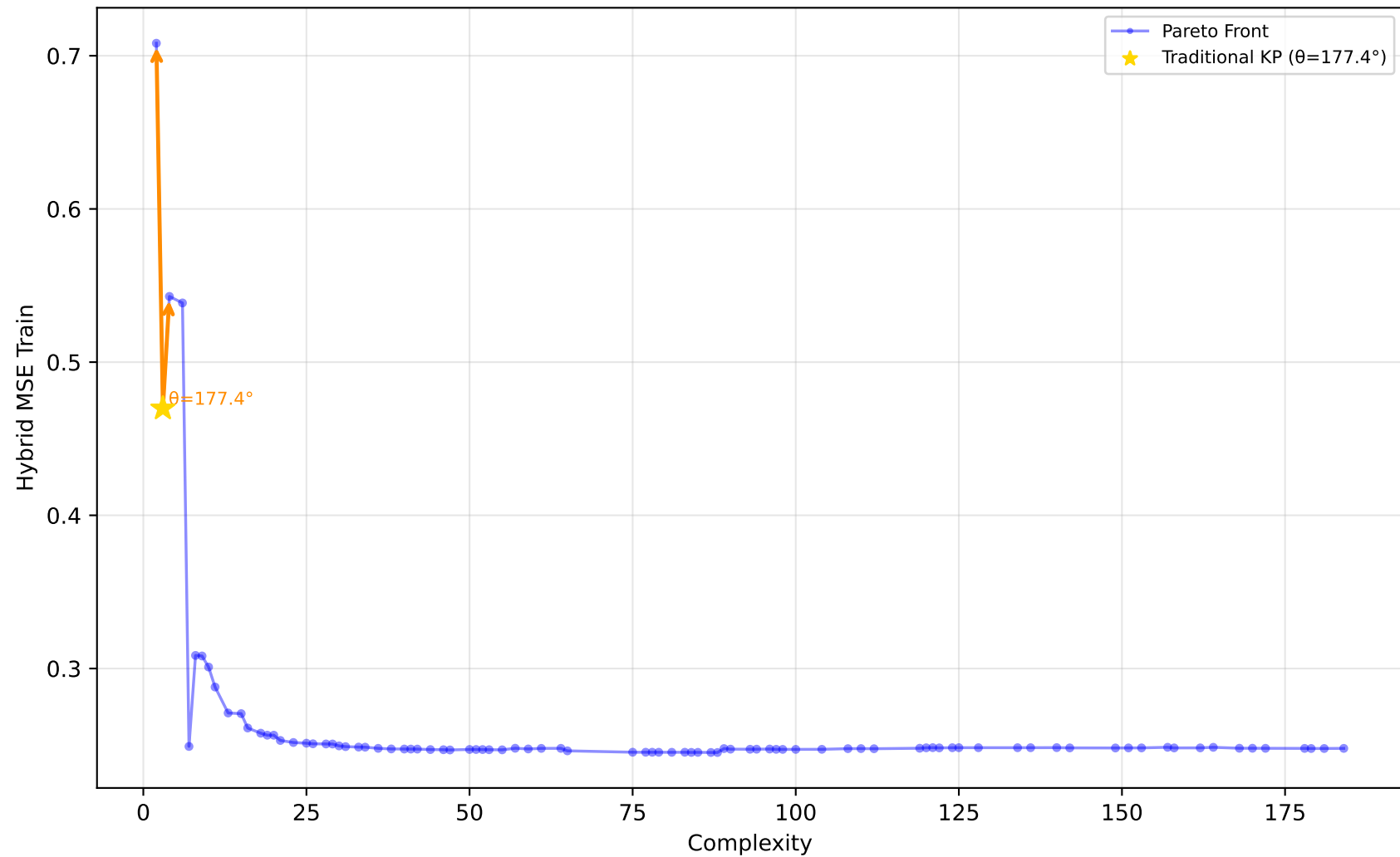
561_cpu - Run 16 - MVP - Hybrid MSE Train \lambda_1=0.50, \lambda_2=0.20, \lambda_3=0.00 | Difficulty: 0.94 | Method: hmr
