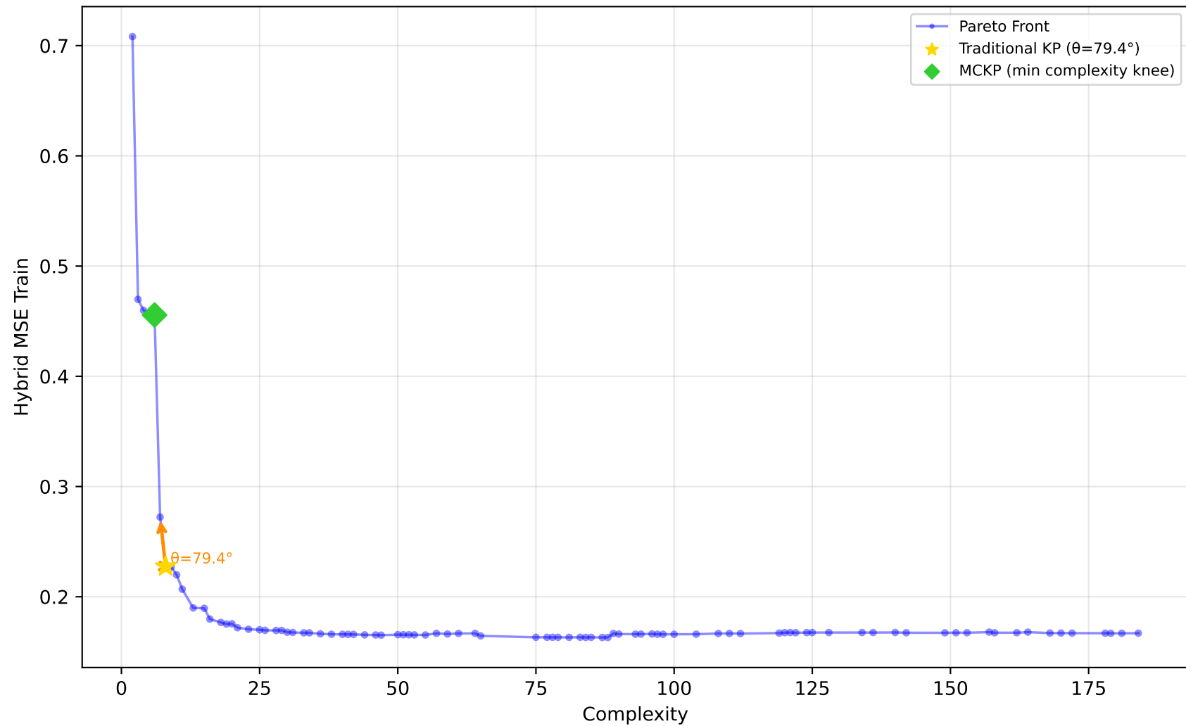
561_cpu - Run 16 - MVP - Hybrid MSE Train \lambda_1=0.70, \lambda_2=0.00, \lambda_3=0.10 | Difficulty: 0.94 | Method: hmr
