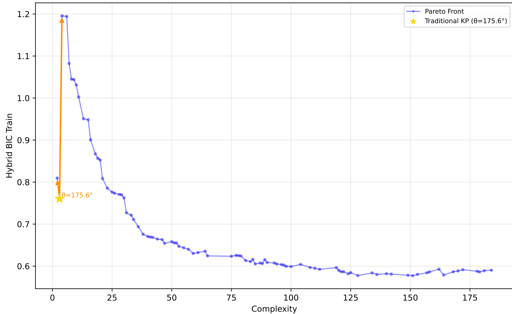
561_cpu - Run 16 - SVP - Hybrid BIC Train \lambda_1=1.00, \lambda_2=0.00, \lambda_3=0.40 | Difficulty: 0.94 | Method: hmr
