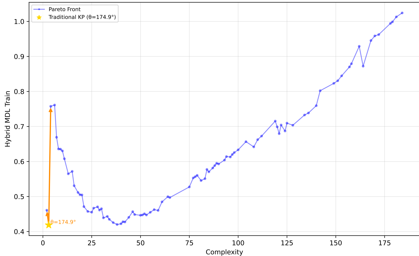
561_cpu - Run 16 - SVP - Hybrid MDL Train \lambda_1=0.90, \lambda_2=0.00, \lambda_3=0.30 | Difficulty: 0.94 | Method: hmr
