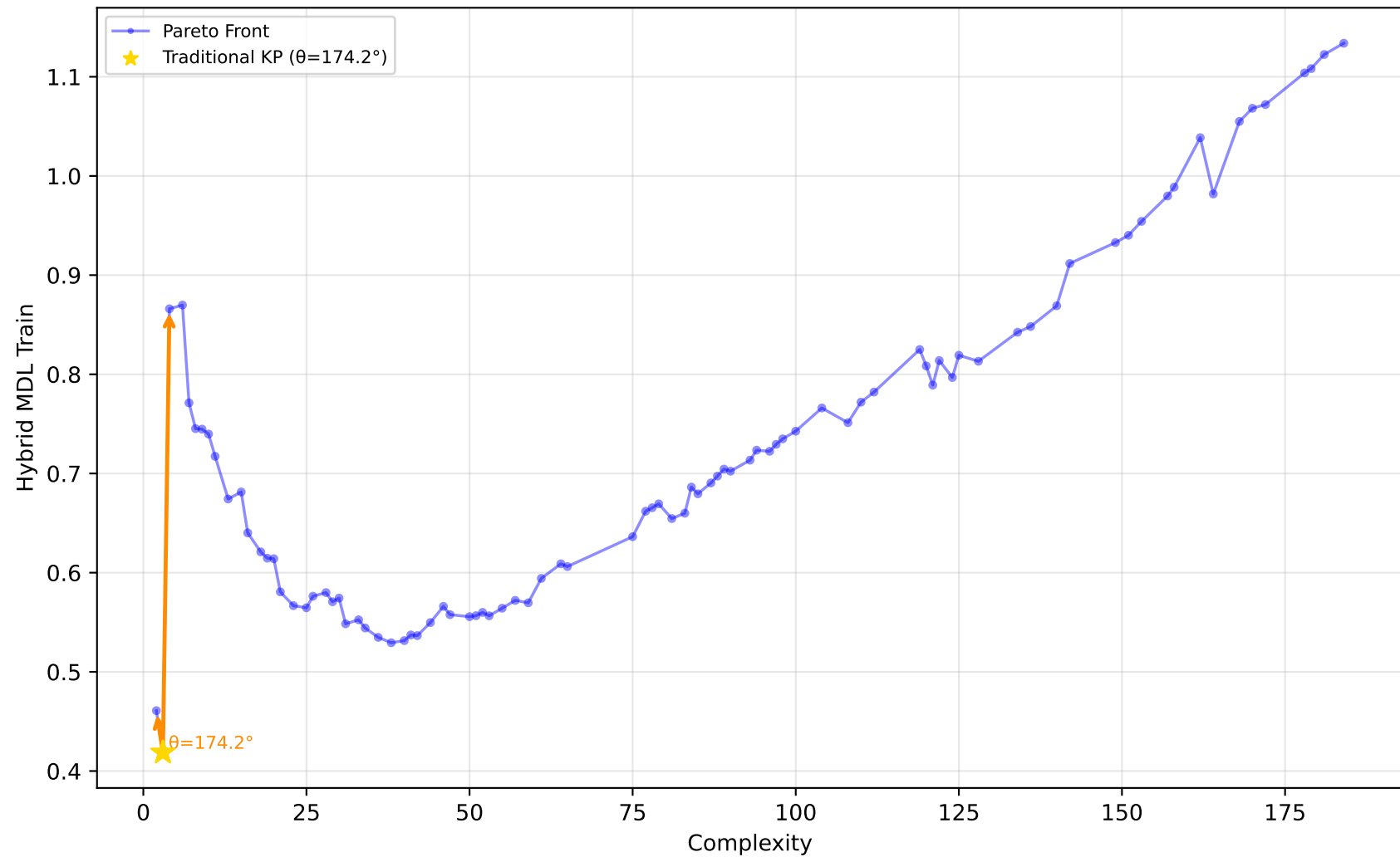
561_cpu - Run 16 - SVP - Hybrid MDL Train \lambda_1=1.00, \lambda_2=0.00, \lambda_3=0.40 | Difficulty: 0.94 | Method: hmr
