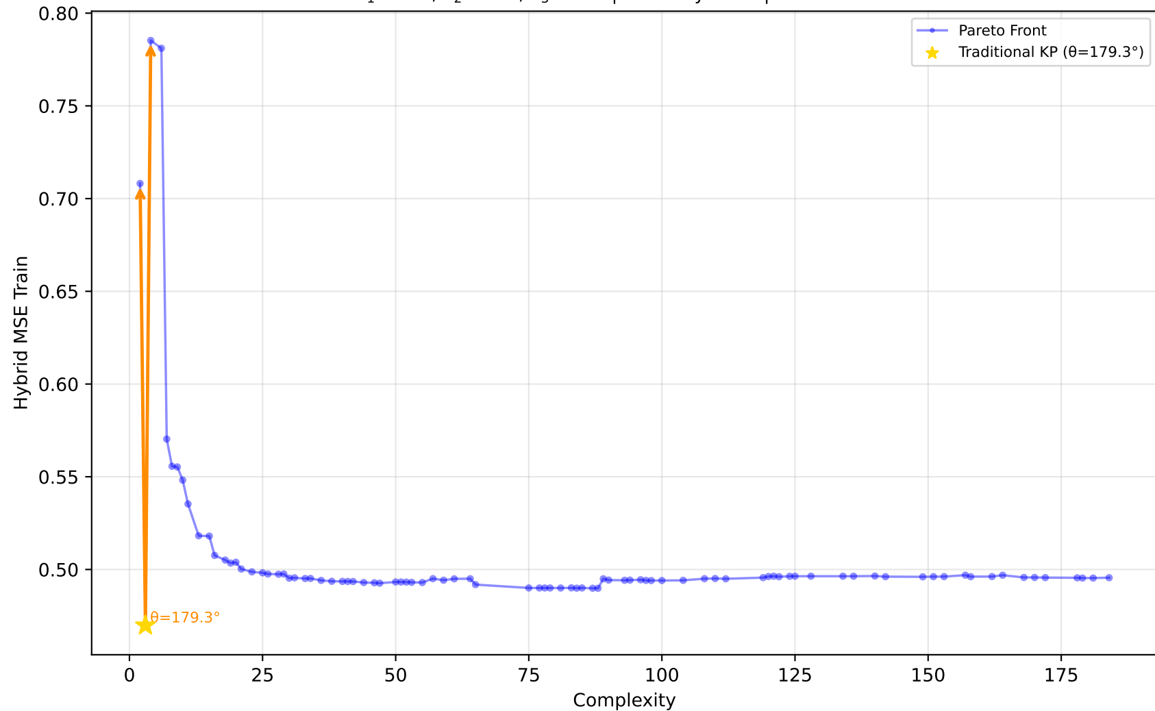
561_cpu - Run 16 - SVP - Hybrid MSE Train \lambda_1=1.00, \lambda_2=0.00, \lambda_3=0.40 | Difficulty: 0.94 | Method: hmr
