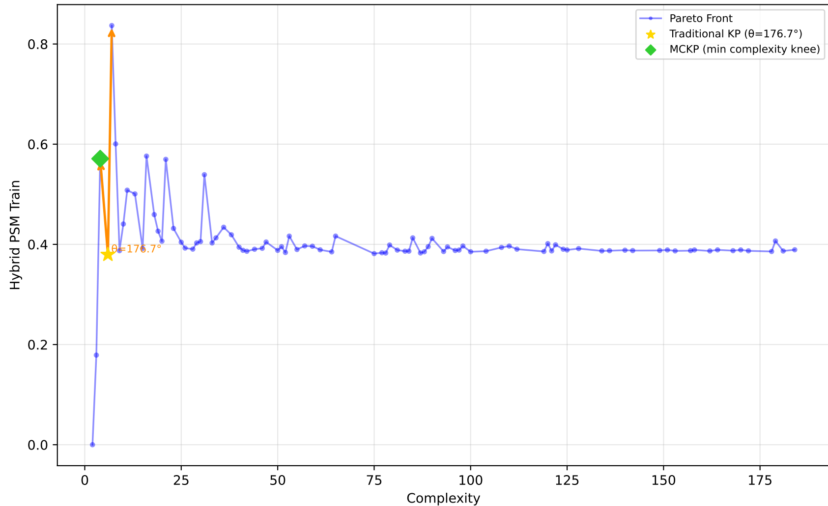
561_cpu - Run 16 - SVP - Hybrid PSM Train \lambda_1=0.90, \lambda_2=0.00, \lambda_3=0.30 | Difficulty: 0.94 | Method: hmr
