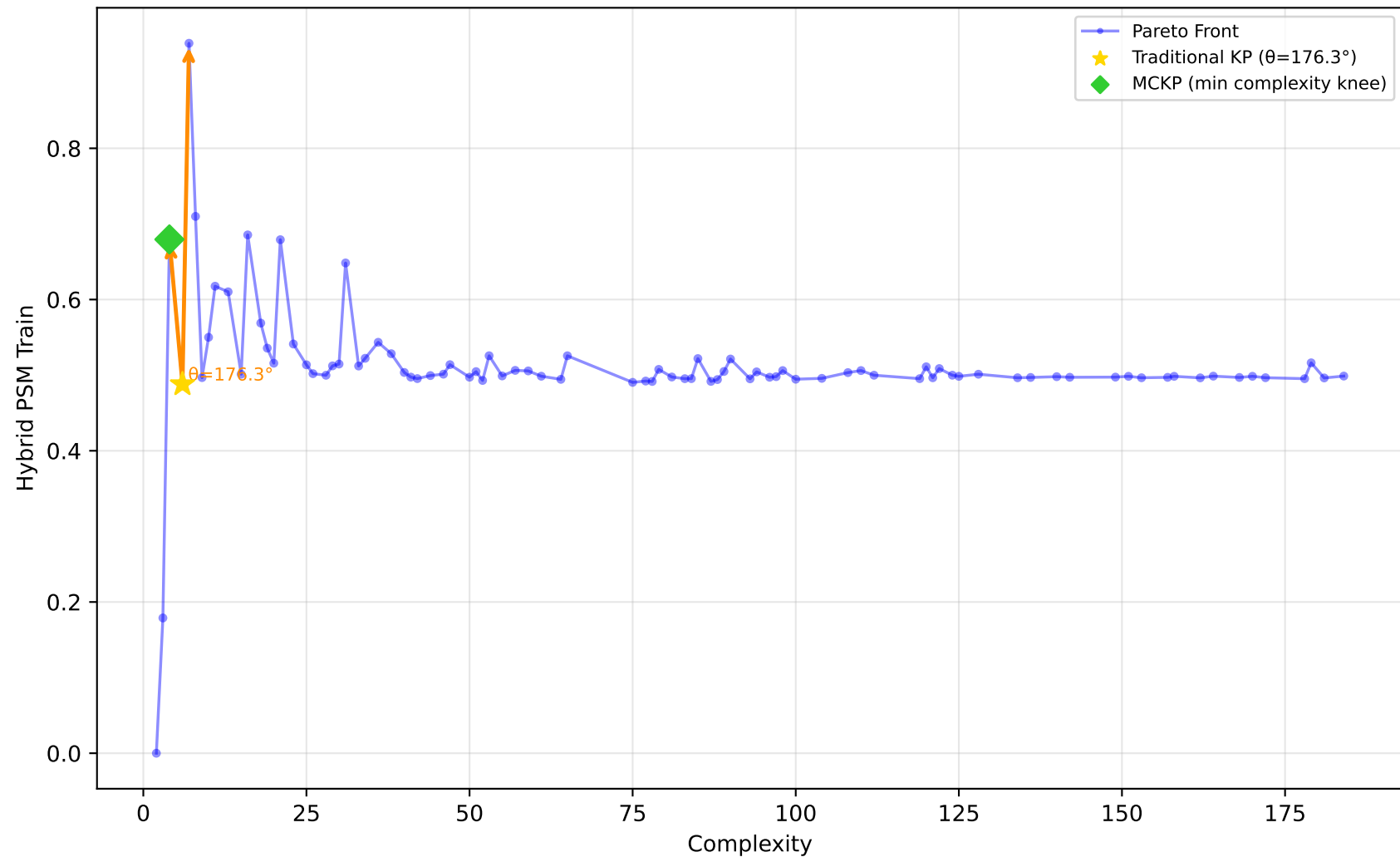
561_cpu - Run 16 - SVP - Hybrid PSM Train \lambda_1=1.00, \lambda_2=0.00, \lambda_3=0.40 | Difficulty: 0.94 | Method: hmr
