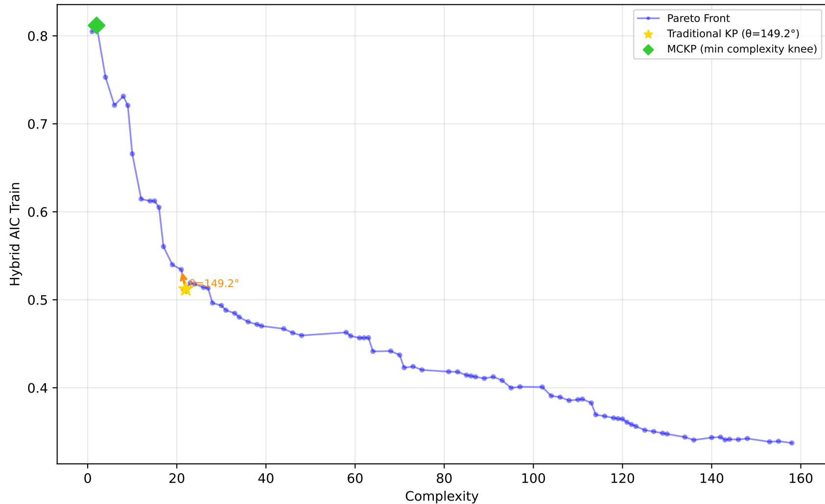
561_cpu - Run 17 - MVP - Hybrid AIC Train \lambda_1=0.70, \lambda_2=0.00, \lambda_3=0.10 | Difficulty: 1.00 | Method: hmr
