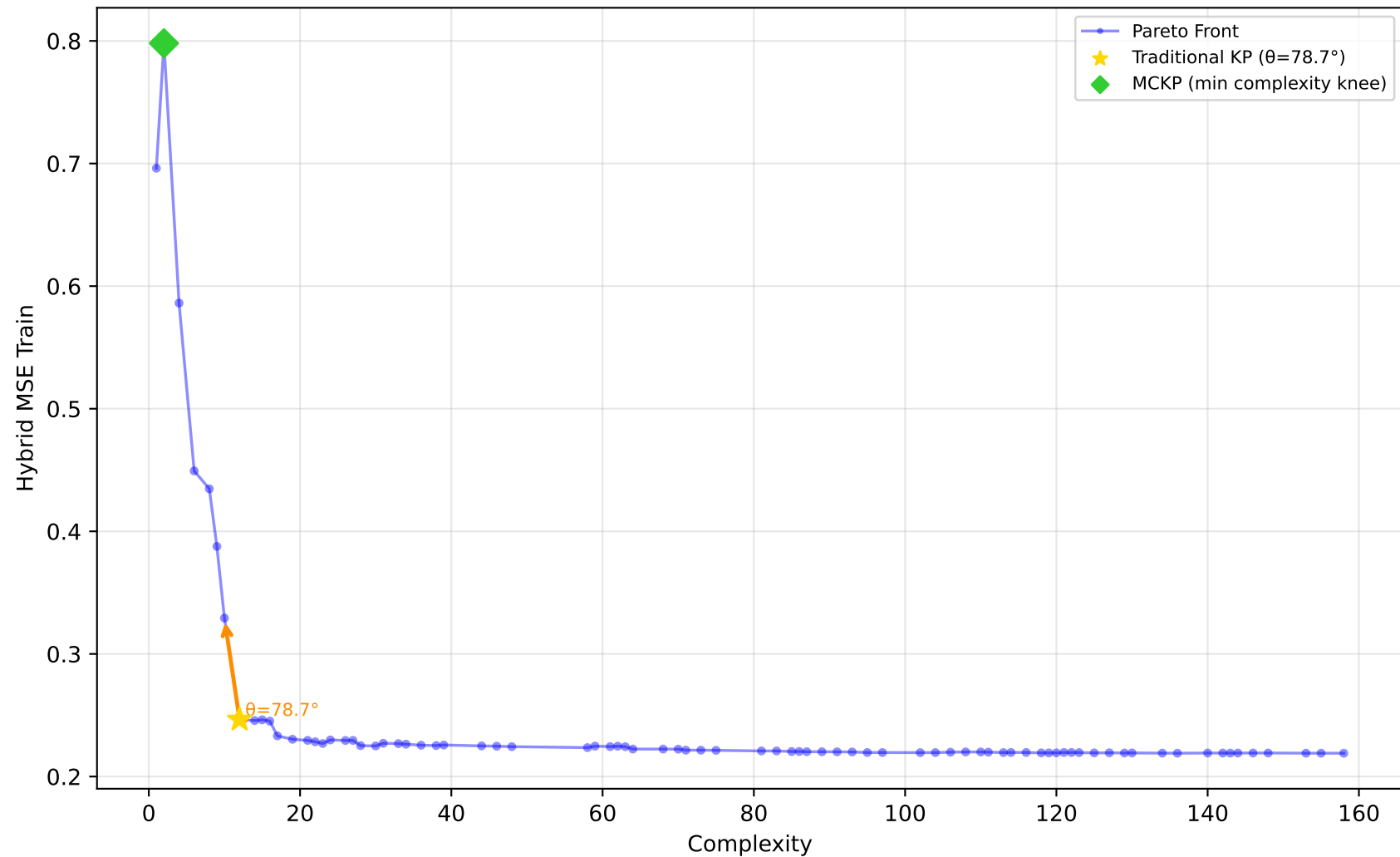
561_cpu - Run 17 - MVP - Hybrid MSE Train \lambda_1=0.50, \lambda_2=0.20, \lambda_3=0.00 | Difficulty: 1.00 | Method: hmr
