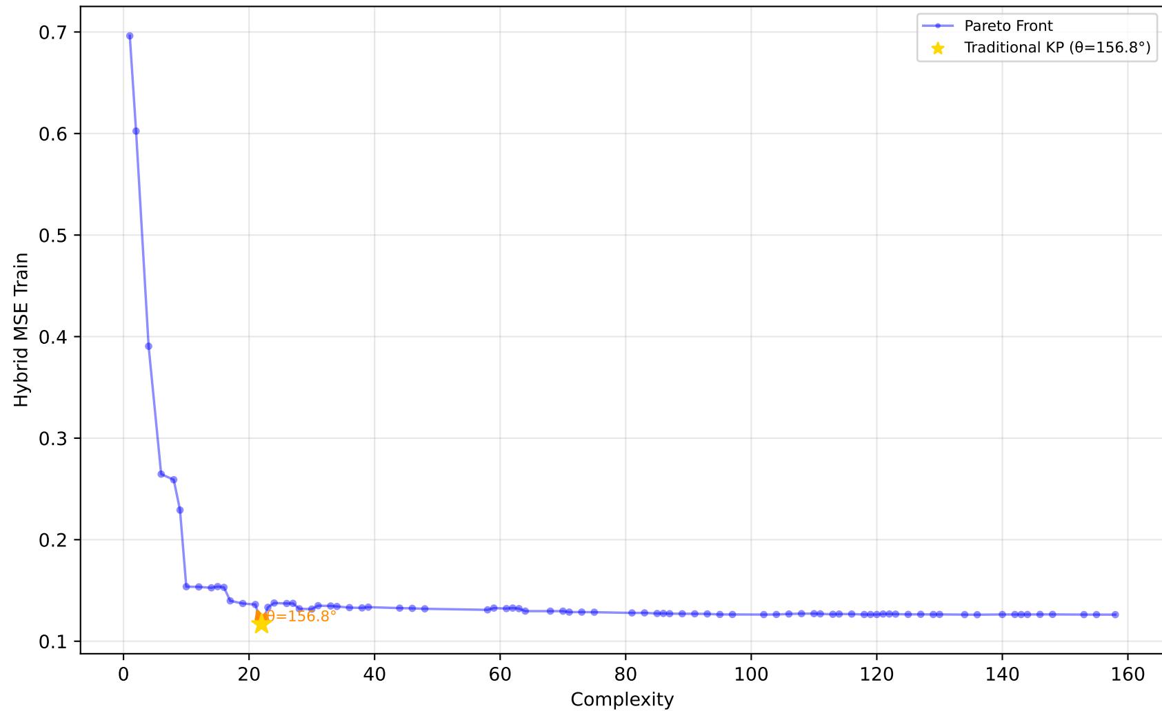
561_cpu - Run 17 - MVP - Hybrid MSE Train \lambda_1=0.70, \lambda_2=0.00, \lambda_3=0.10 | Difficulty: 1.00 | Method: hmr
