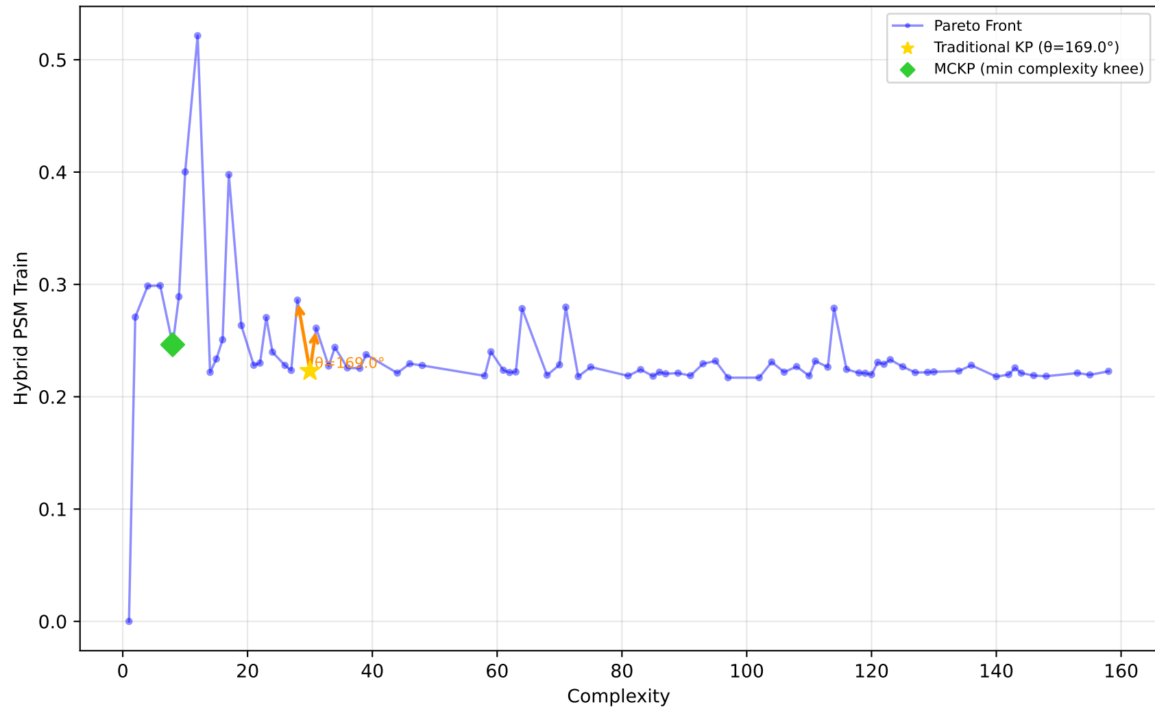
561_cpu - Run 17 - MVP - Hybrid PSM Train \lambda_1=0.50, \lambda_2=0.20, \lambda_3=0.00 | Difficulty: 1.00 | Method: hmr
