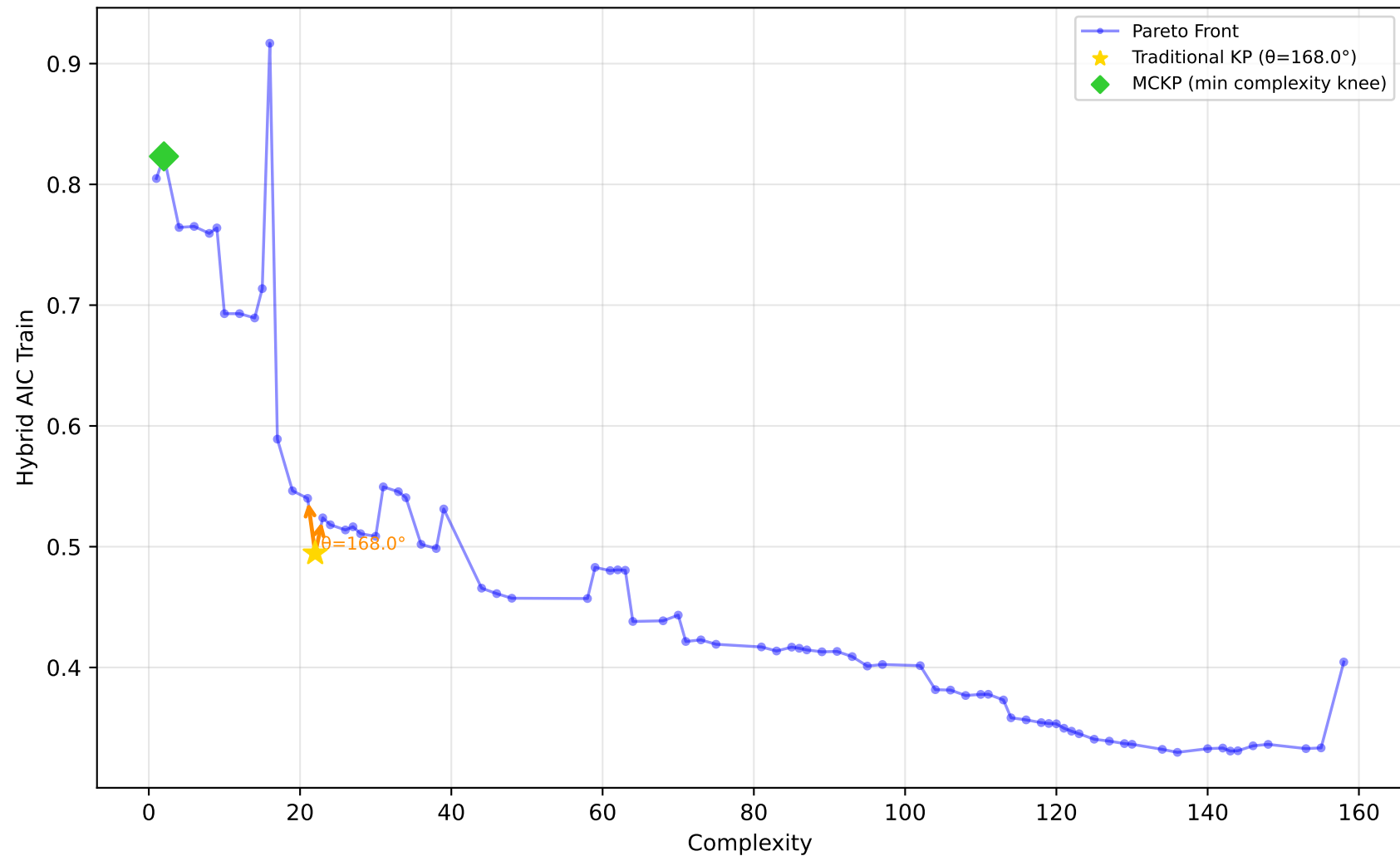
561_cpu - Run 17 - SVP - Hybrid AIC Train \lambda_1=1.00, \lambda_2=0.00, \lambda_3=0.40 | Difficulty: 1.00 | Method: hmr
