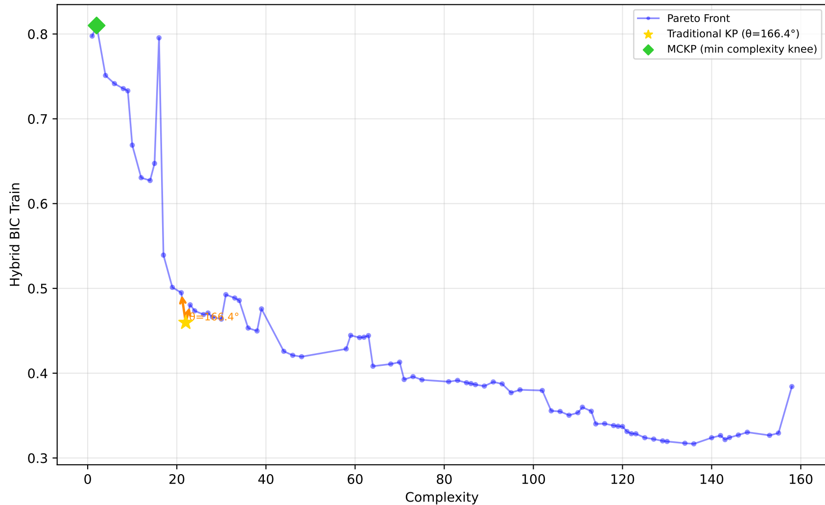
561_cpu - Run 17 - SVP - Hybrid BIC Train \lambda_1=0.90, \lambda_2=0.00, \lambda_3=0.30 | Difficulty: 1.00 | Method: hmr
