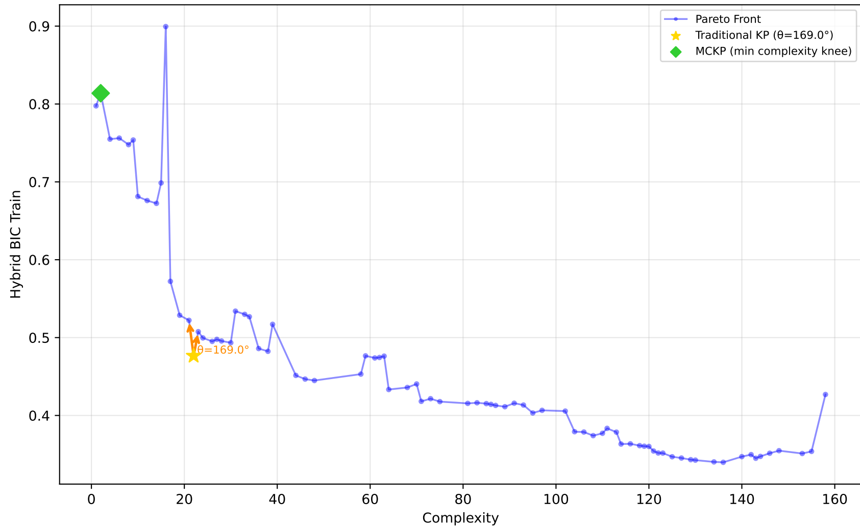
561_cpu - Run 17 - SVP - Hybrid BIC Train \lambda_1=1.00, \lambda_2=0.00, \lambda_3=0.40 | Difficulty: 1.00 | Method: hmr
