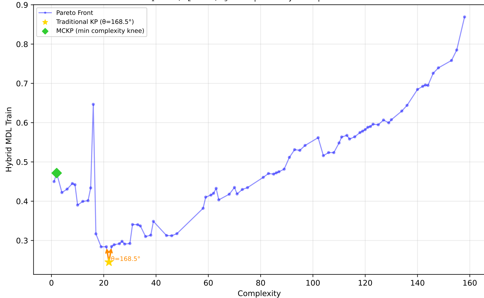
561_cpu - Run 17 - SVP - Hybrid MDL Train \lambda_1=1.00, \lambda_2=0.00, \lambda_3=0.40 | Difficulty: 1.00 | Method: hmr
