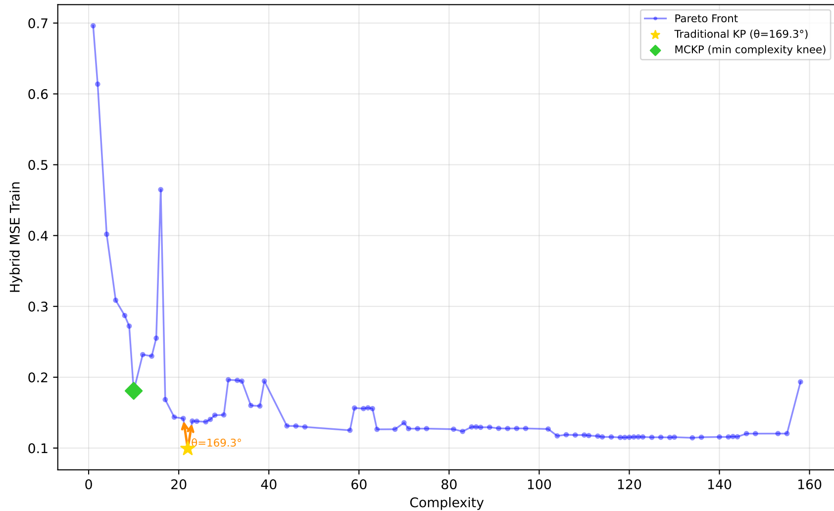
561_cpu - Run 17 - SVP - Hybrid MSE Train \lambda_1=1.00, \lambda_2=0.00, \lambda_3=0.40 | Difficulty: 1.00 | Method: hmr
