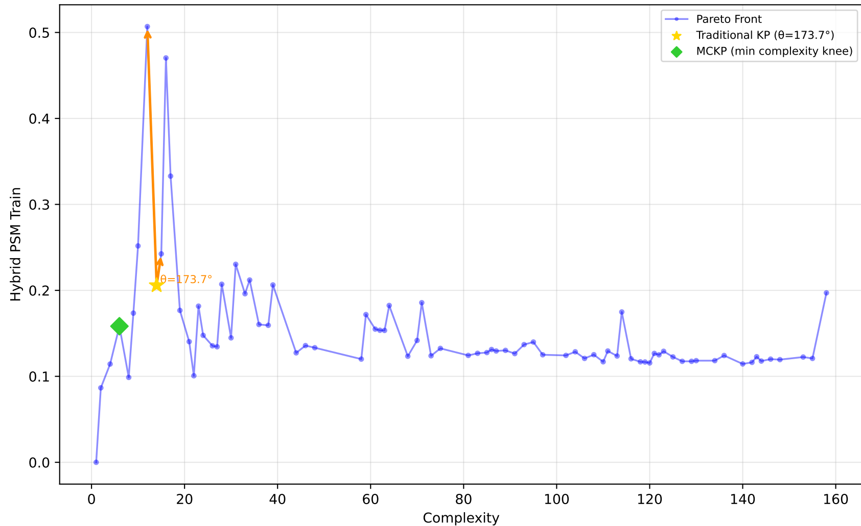
561_cpu - Run 17 - SVP - Hybrid PSM Train \lambda_1=1.00, \lambda_2=0.00, \lambda_3=0.40 | Difficulty: 1.00 | Method: hmr
