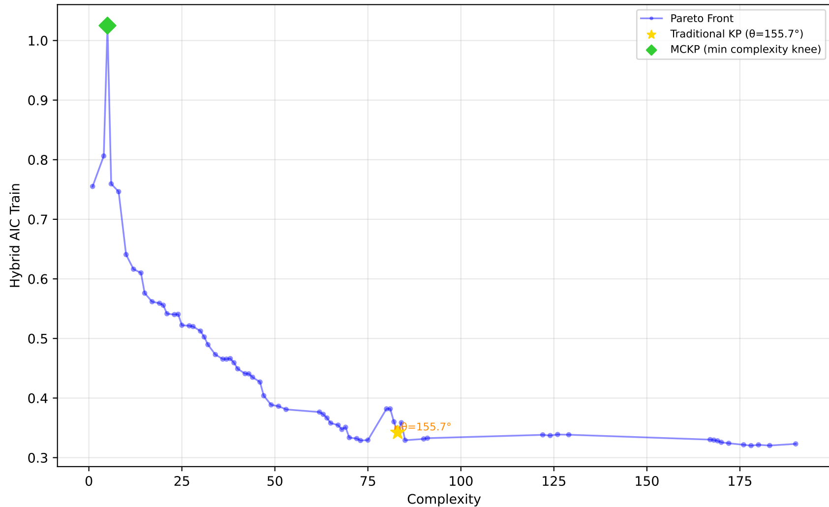
561_cpu - Run 18 - MVP - Hybrid AIC Train \lambda_1=0.50, \lambda_2=0.20, \lambda_3=0.00 | Difficulty: 1.00 | Method: hmr
