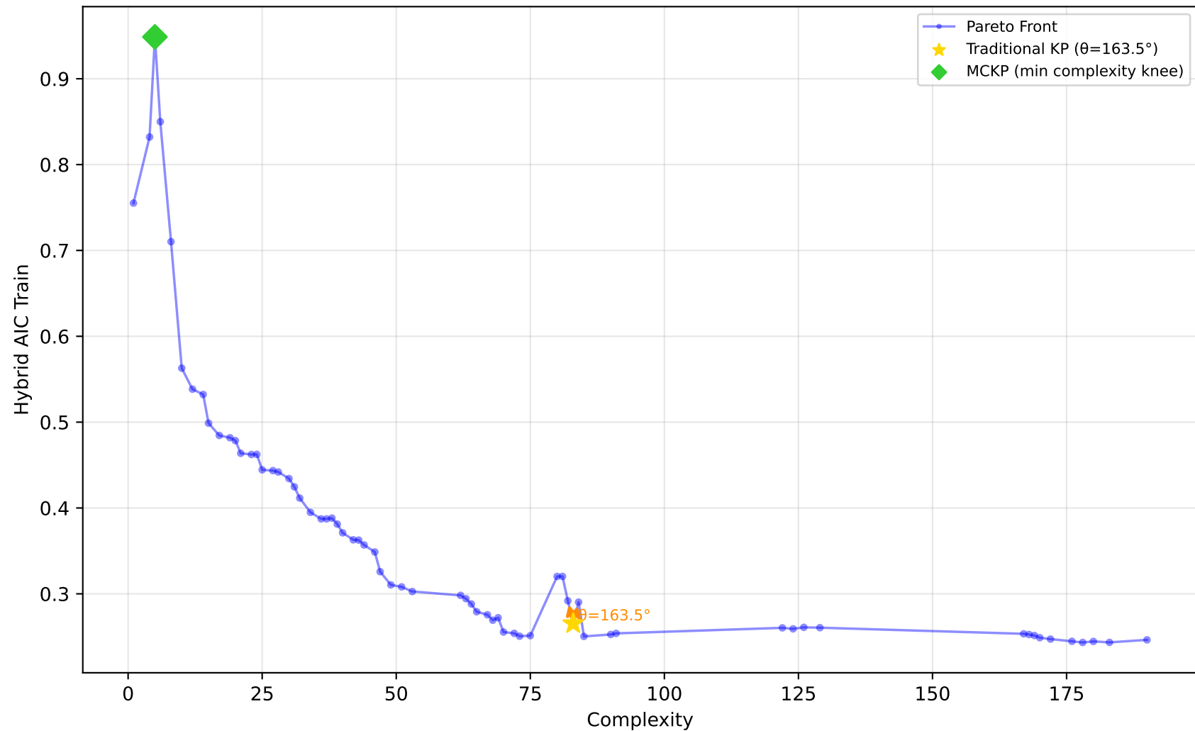
561_cpu - Run 18 - MVP - Hybrid AIC Train \lambda_1=0.70, \lambda_2=0.00, \lambda_3=0.10 | Difficulty: 1.00 | Method: hmr
