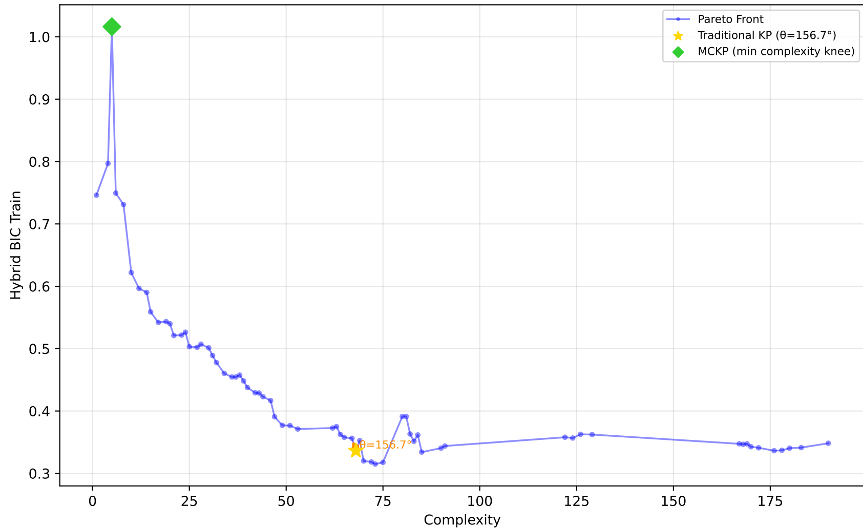
561_cpu - Run 18 - MVP - Hybrid BIC Train \lambda_1=0.50, \lambda_2=0.20, \lambda_3=0.00 | Difficulty: 1.00 | Method: hmr
