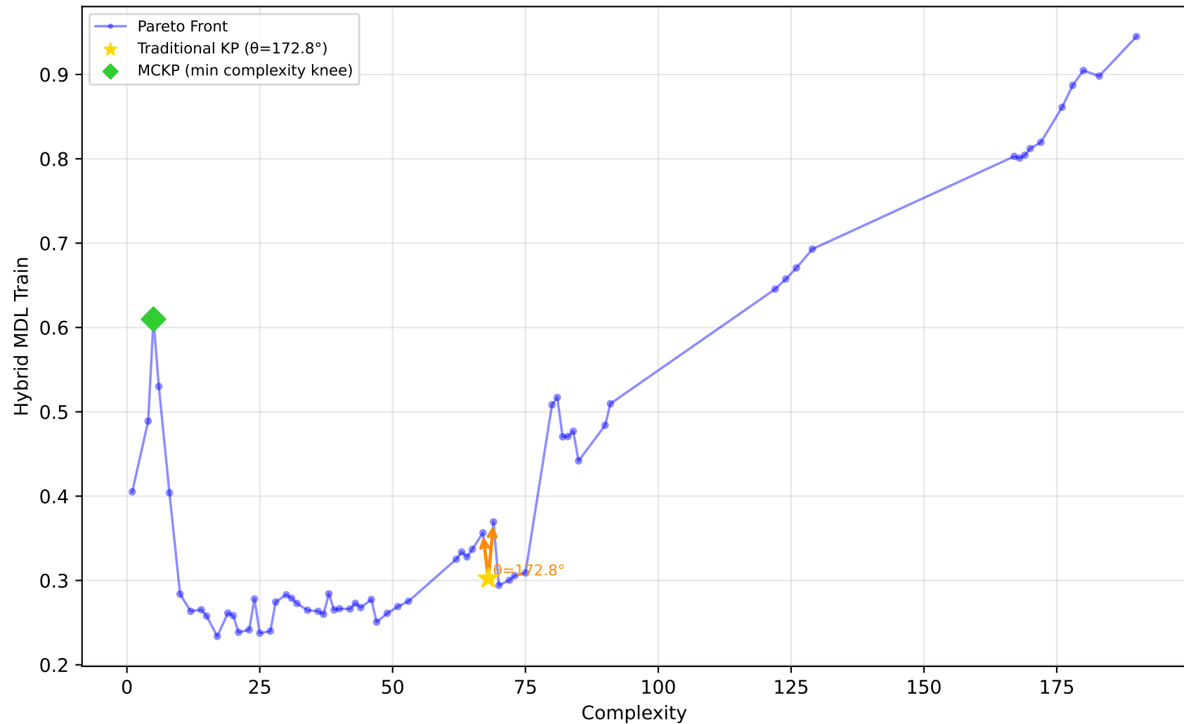
561_cpu - Run 18 - MVP - Hybrid MDL Train \lambda_1=0.70, \lambda_2=0.00, \lambda_3=0.10 | Difficulty: 1.00 | Method: hmr
