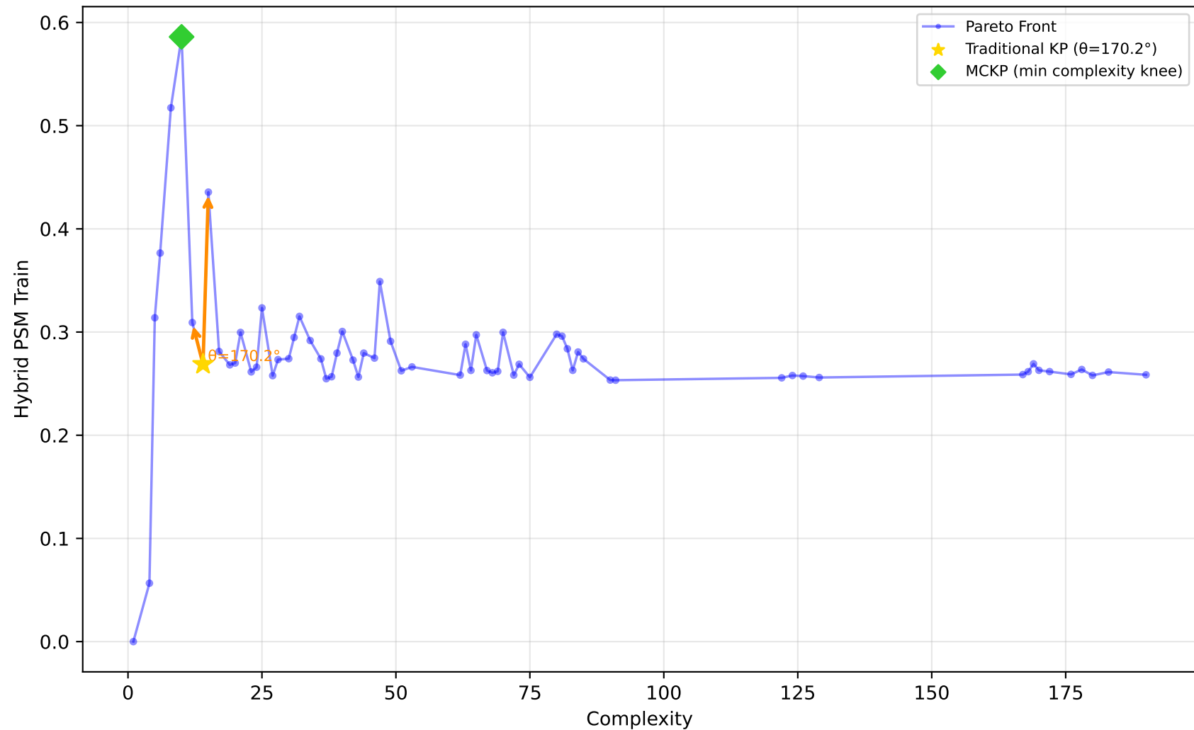
561_cpu - Run 18 - MVP - Hybrid PSM Train \lambda_1=0.50, \lambda_2=0.20, \lambda_3=0.00 | Difficulty: 1.00 | Method: hmr
