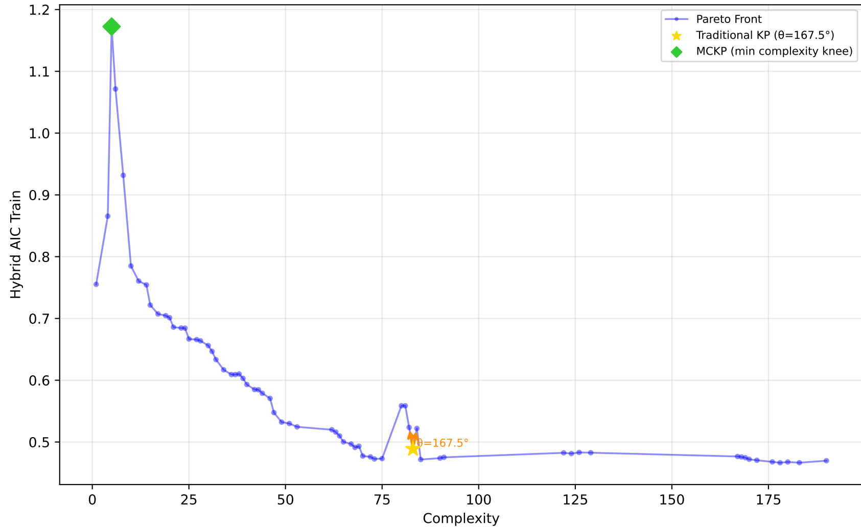
561_cpu - Run 18 - SVP - Hybrid AIC Train \lambda_1=0.90, \lambda_2=0.00, \lambda_3=0.30 | Difficulty: 1.00 | Method: hmr
