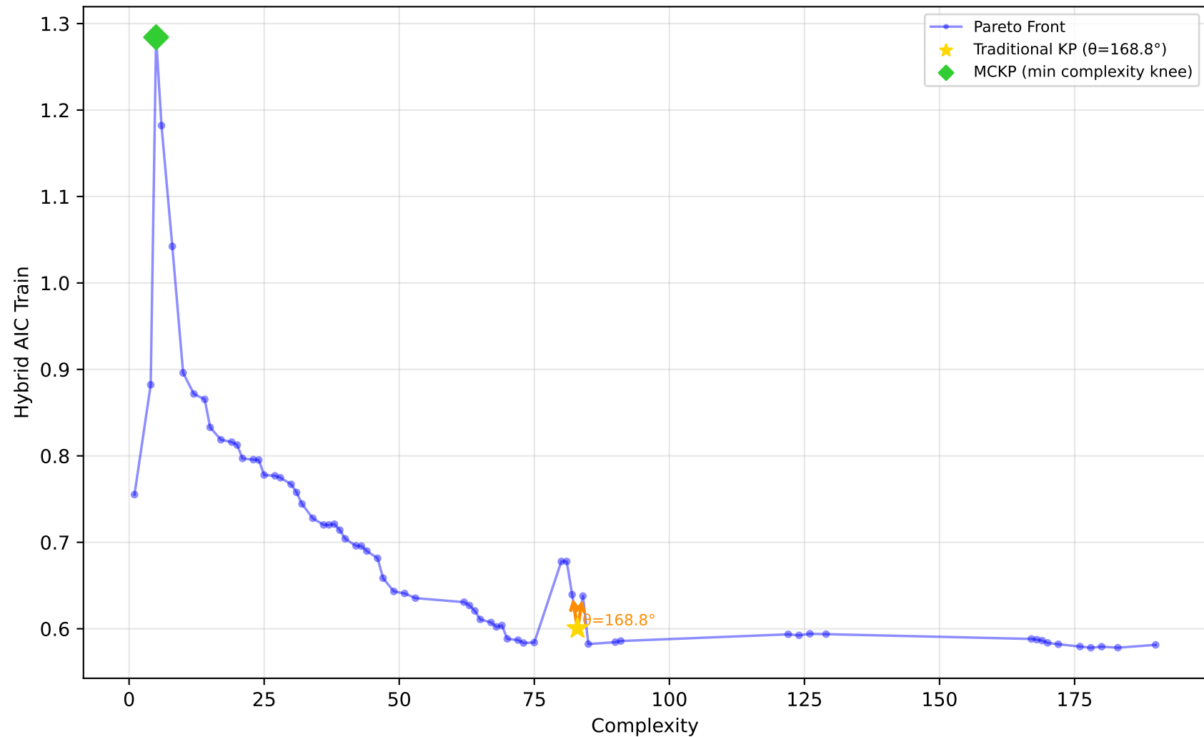
561_cpu - Run 18 - SVP - Hybrid AIC Train \lambda_1=1.00, \lambda_2=0.00, \lambda_3=0.40 | Difficulty: 1.00 | Method: hmr
