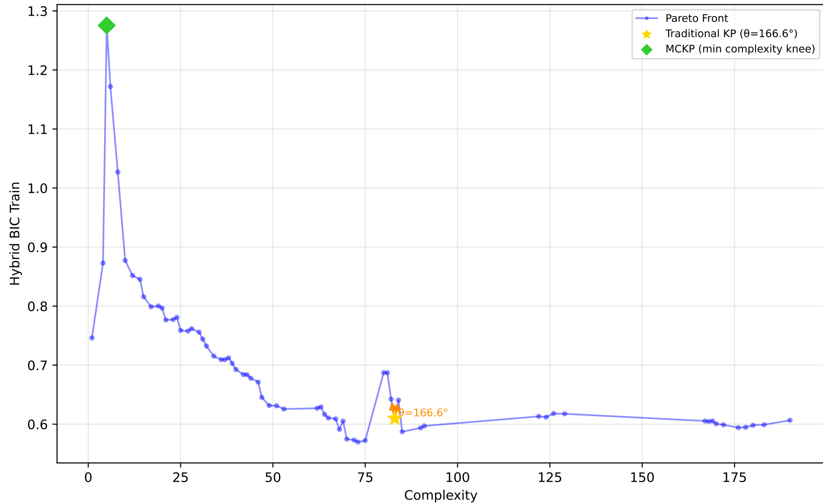
561_cpu - Run 18 - SVP - Hybrid BIC Train \lambda_1=1.00, \lambda_2=0.00, \lambda_3=0.40 | Difficulty: 1.00 | Method: hmr
