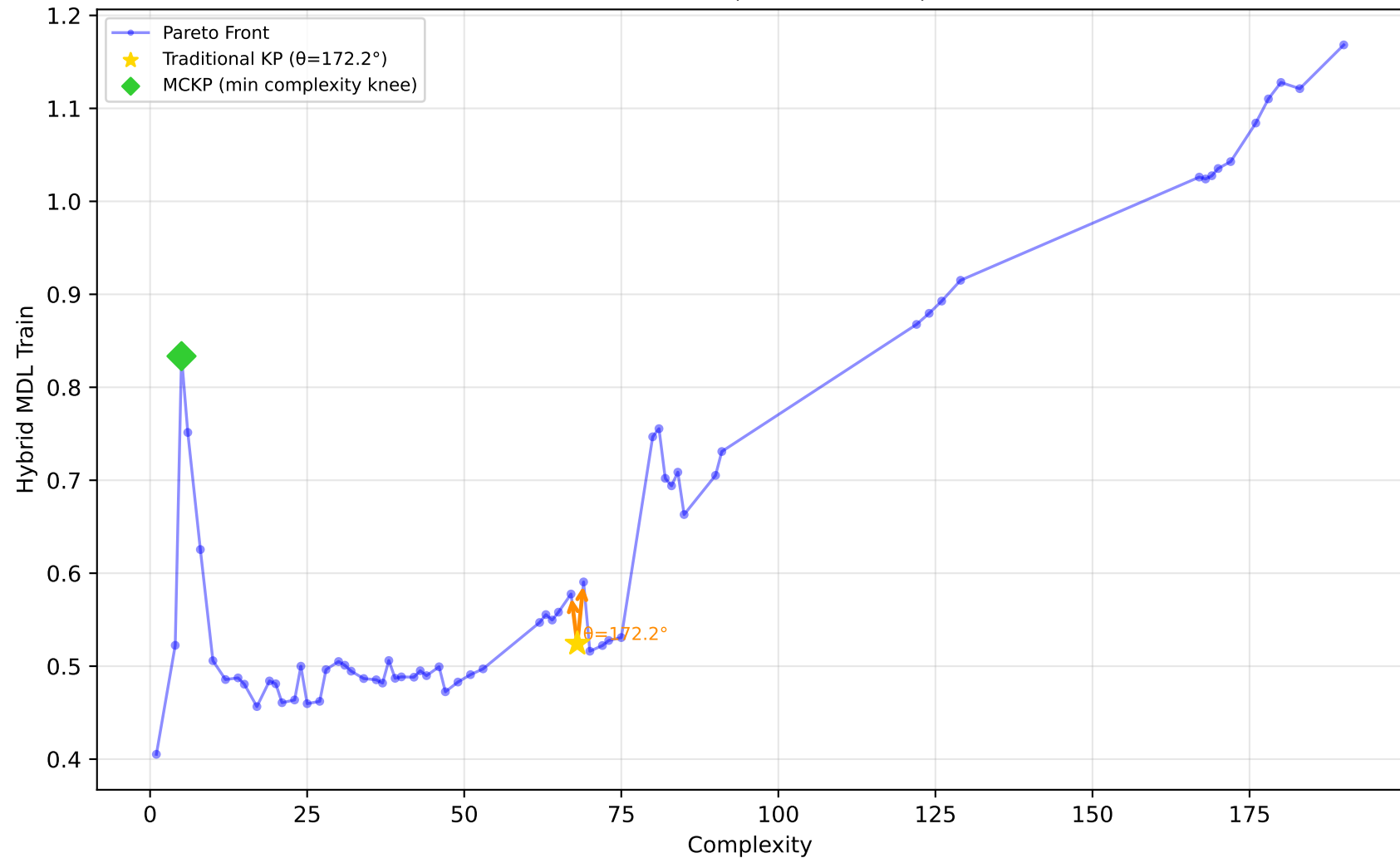
561_cpu - Run 18 - SVP - Hybrid MDL Train \lambda_1=0.90, \lambda_2=0.00, \lambda_3=0.30 | Difficulty: 1.00 | Method: hmr
