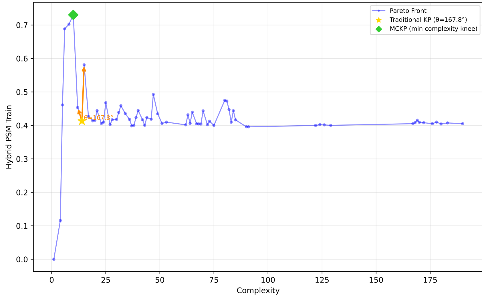
561_cpu - Run 18 - SVP - Hybrid PSM Train \lambda_1=0.90, \lambda_2=0.00, \lambda_3=0.30 | Difficulty: 1.00 | Method: hmr
