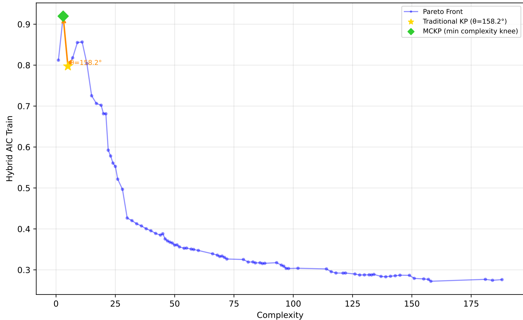
561_cpu - Run 19 - MVP - Hybrid AIC Train \lambda_1=0.50, \lambda_2=0.20, \lambda_3=0.00 | Difficulty: 1.00 | Method: hmr
