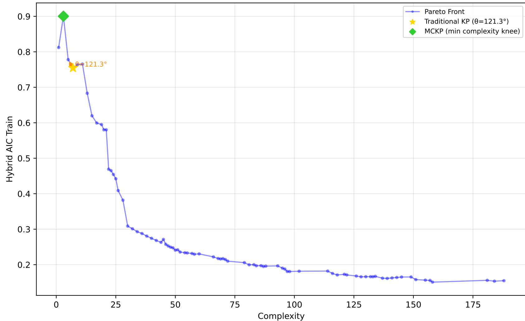
561_cpu - Run 19 - MVP - Hybrid AIC Train \lambda_1=0.70, \lambda_2=0.00, \lambda_3=0.10 | Difficulty: 1.00 | Method: hmr
