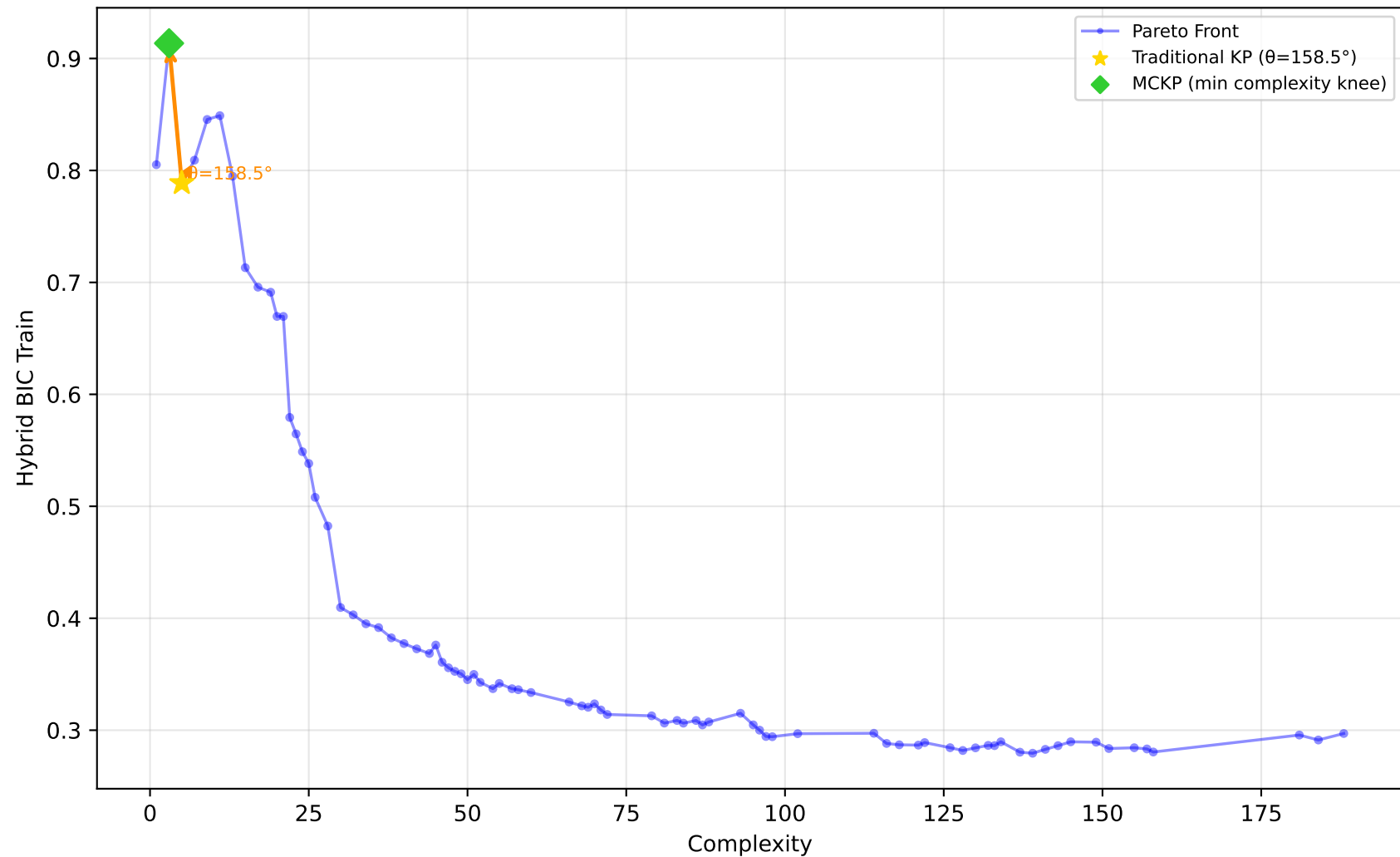
561_cpu - Run 19 - MVP - Hybrid BIC Train \lambda_1=0.50, \lambda_2=0.20, \lambda_3=0.00 | Difficulty: 1.00 | Method: hmr
