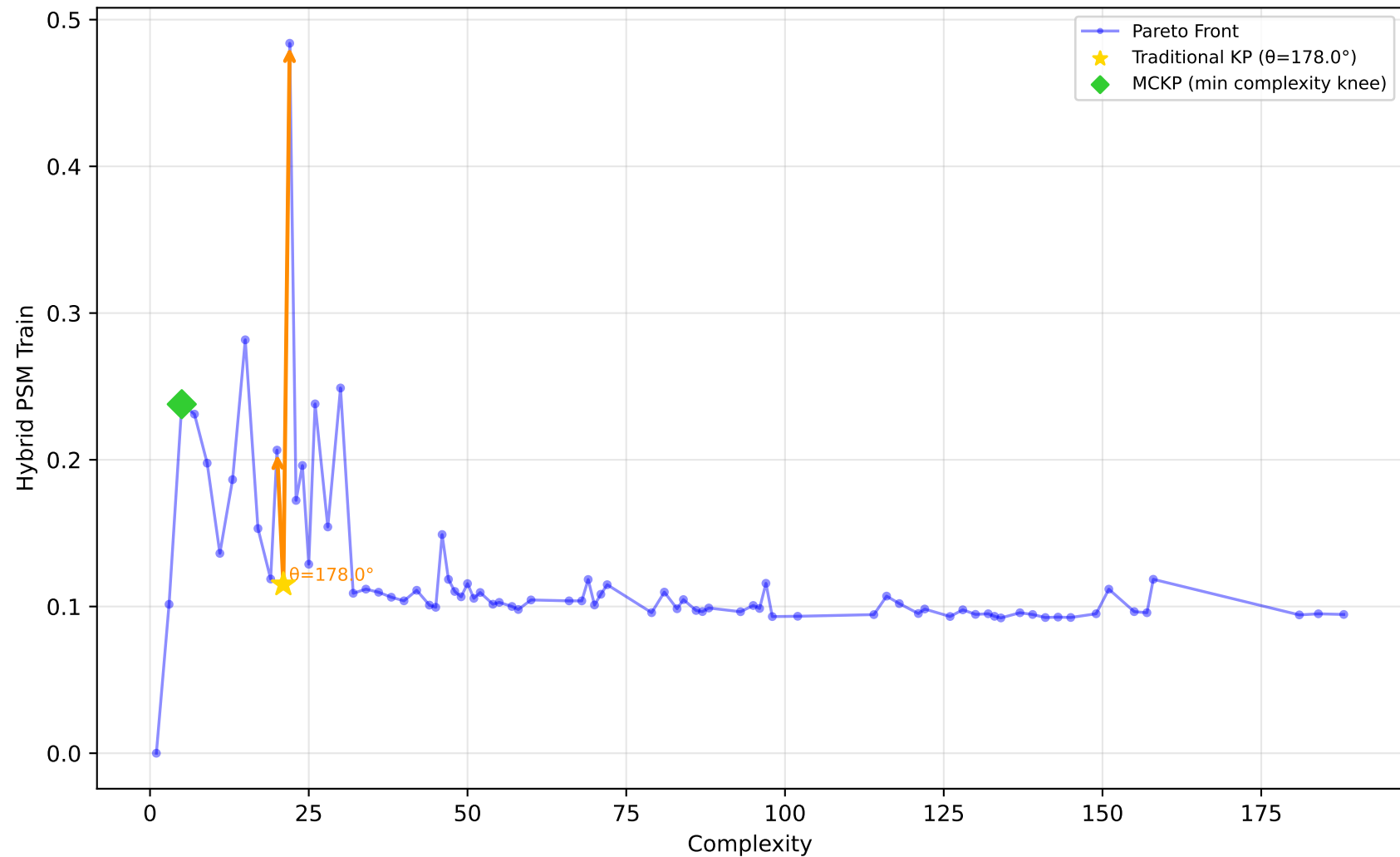
561_cpu - Run 19 - MVP - Hybrid PSM Train \lambda_1=0.70, \lambda_2=0.00, \lambda_3=0.10 | Difficulty: 1.00 | Method: hmr
