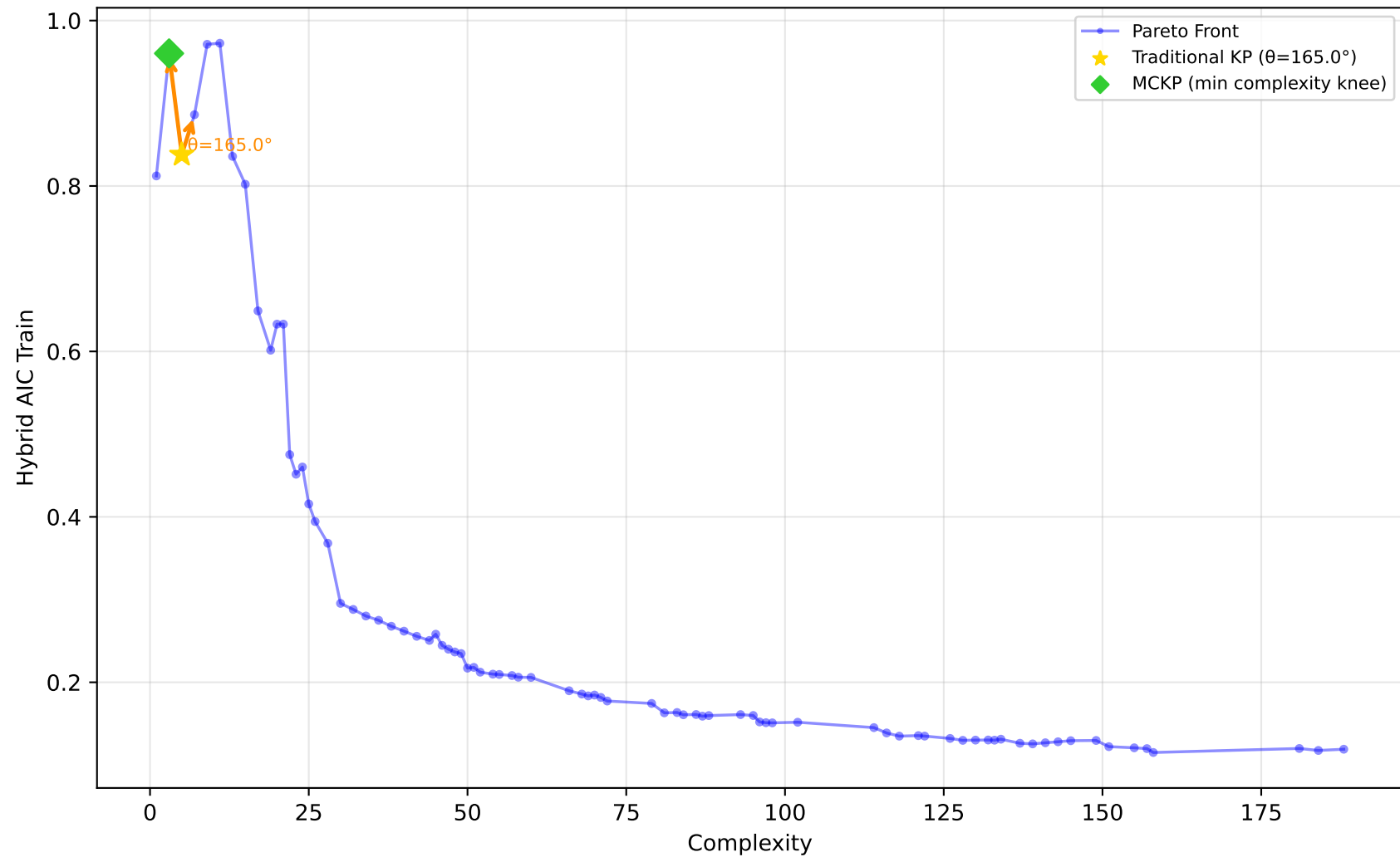
561_cpu - Run 19 - SVP - Hybrid AIC Train \lambda_1=0.90, \lambda_2=0.00, \lambda_3=0.30 | Difficulty: 1.00 | Method: hmr
