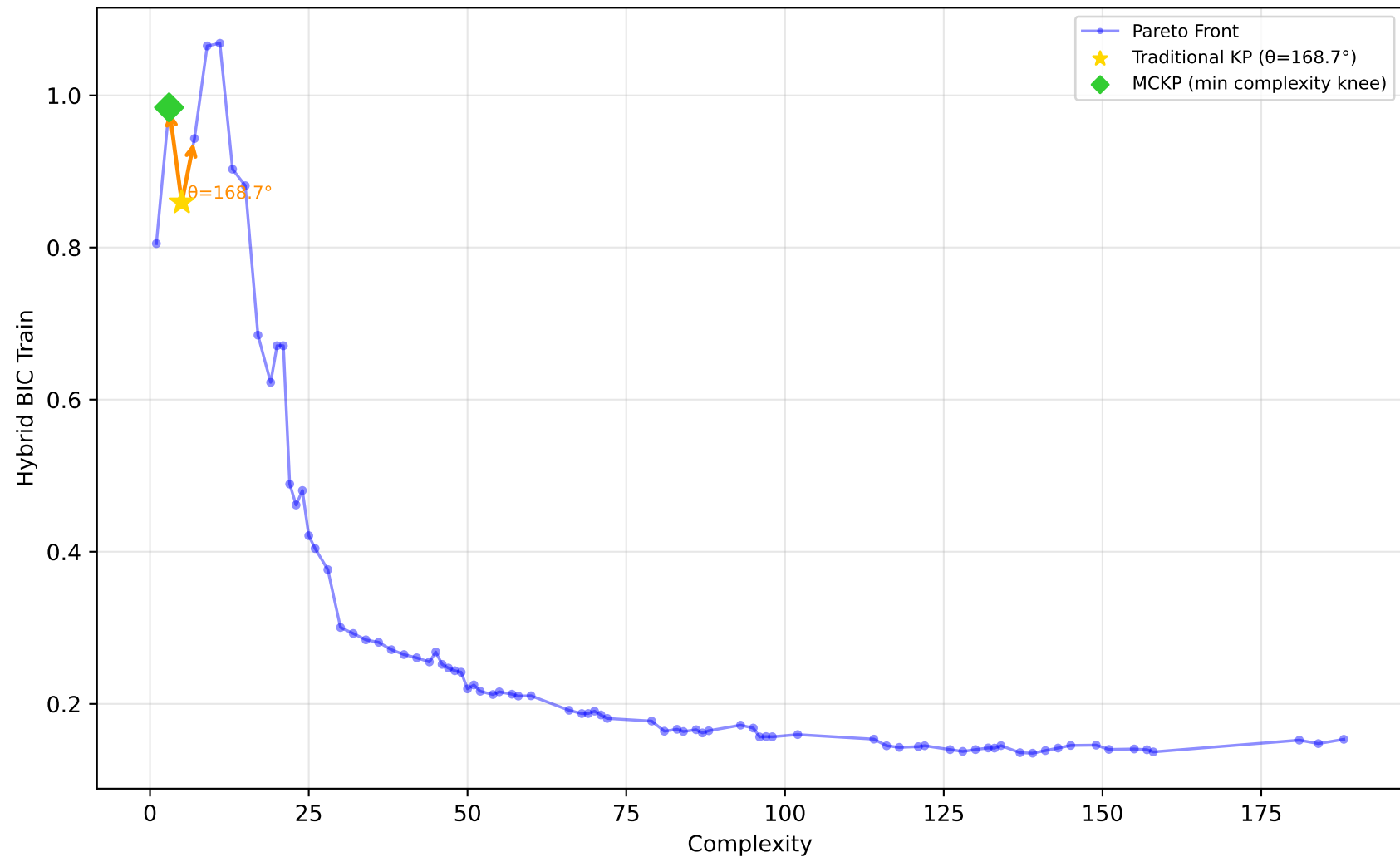
561_cpu - Run 19 - SVP - Hybrid BIC Train \lambda_1=1.00, \lambda_2=0.00, \lambda_3=0.40 | Difficulty: 1.00 | Method: hmr
