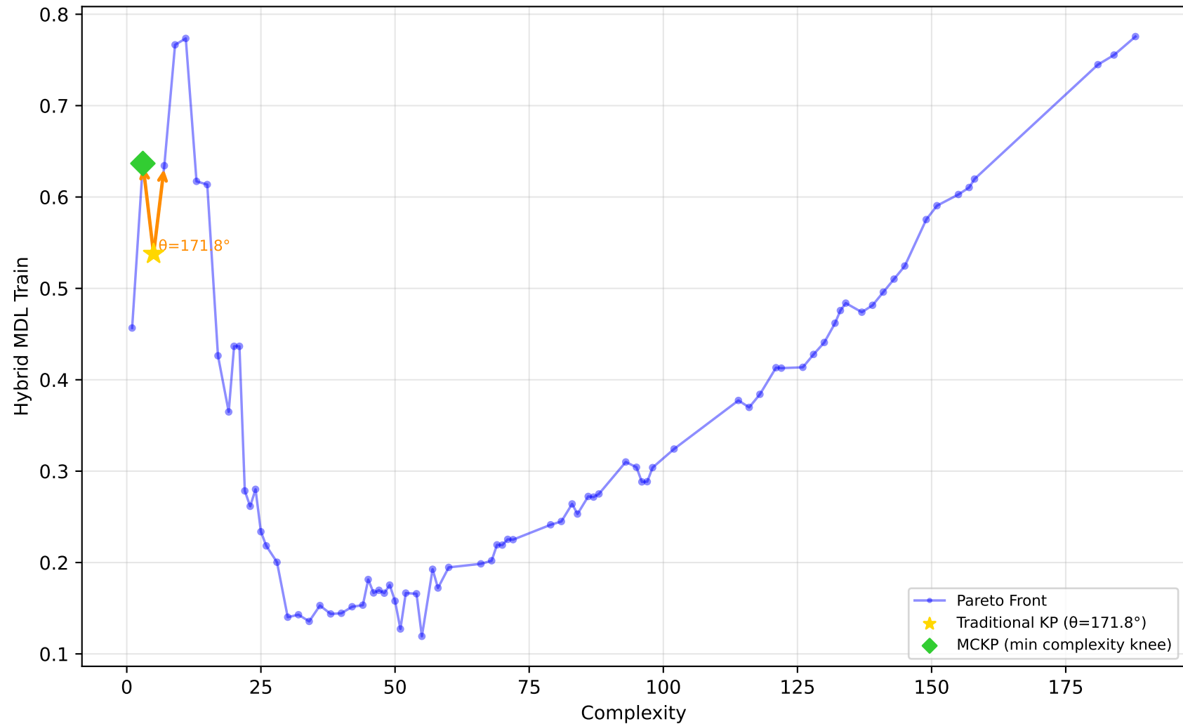
561_cpu - Run 19 - SVP - Hybrid MDL Train \lambda_1=1.00, \lambda_2=0.00, \lambda_3=0.40 | Difficulty: 1.00 | Method: hmr
