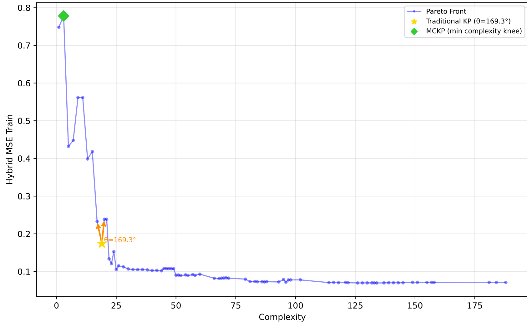
561_cpu - Run 19 - SVP - Hybrid MSE Train \lambda_1=1.00, \lambda_2=0.00, \lambda_3=0.40 | Difficulty: 1.00 | Method: hmr
