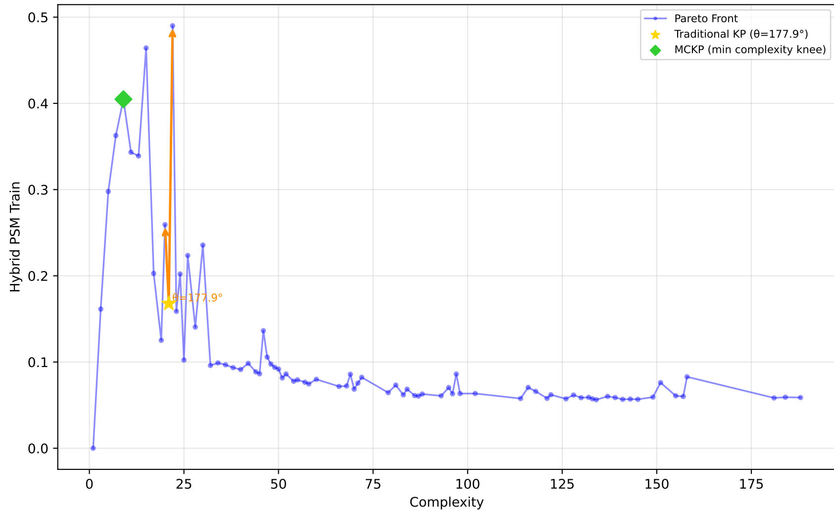
561_cpu - Run 19 - SVP - Hybrid PSM Train \lambda_1=0.90, \lambda_2=0.00, \lambda_3=0.30 | Difficulty: 1.00 | Method: hmr
