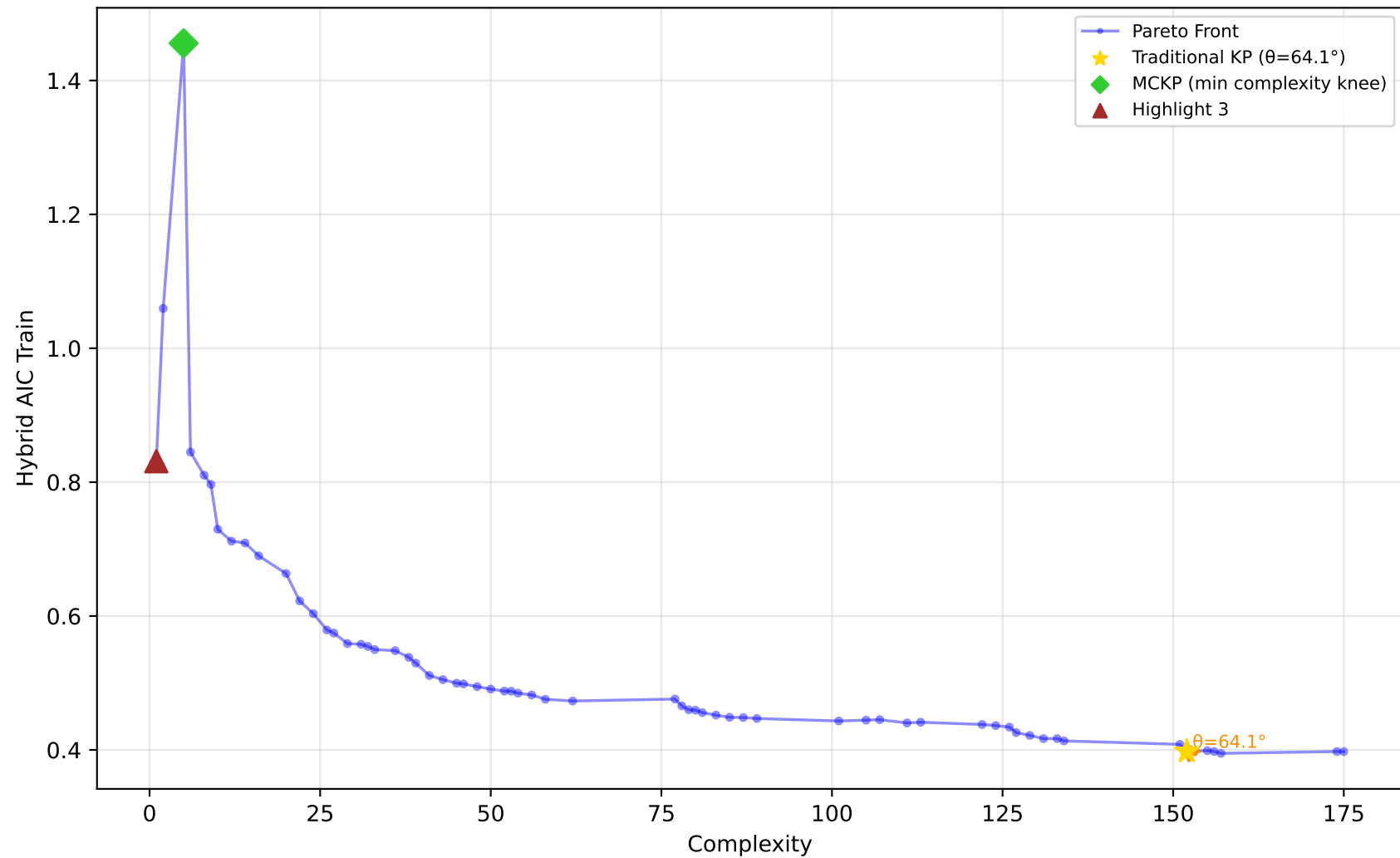
561_cpu - Run 1 - MVP - Hybrid AIC Train \lambda_1=0.50, \lambda_2=0.20, \lambda_3=0.00 | Difficulty: 0.94 | Method: hmr
