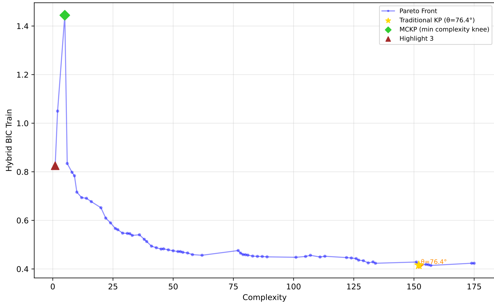
561_cpu - Run 1 - MVP - Hybrid BIC Train \lambda_1=0.50, \lambda_2=0.20, \lambda_3=0.00 | Difficulty: 0.94 | Method: hmr
