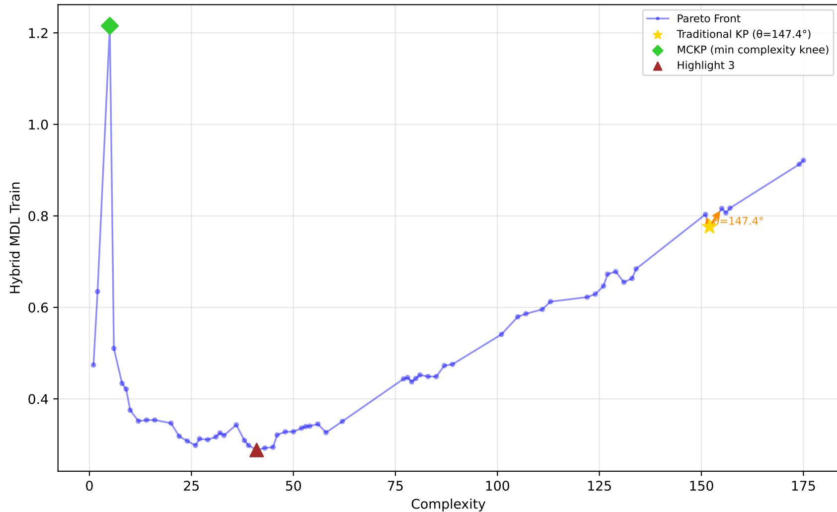
561_cpu - Run 1 - MVP - Hybrid MDL Train \lambda_1=0.70, \lambda_2=0.00, \lambda_3=0.10 | Difficulty: 0.94 | Method: hmr
