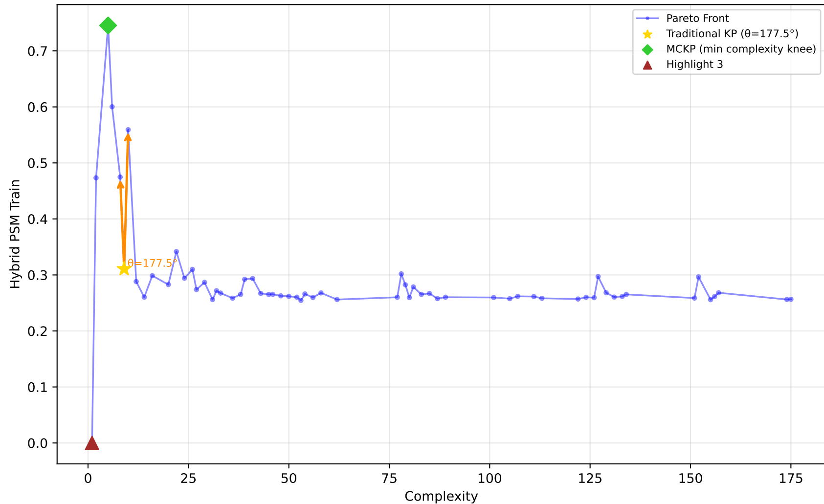
561_cpu - Run 1 - MVP - Hybrid PSM Train \lambda_1=0.50, \lambda_2=0.20, \lambda_3=0.00 | Difficulty: 0.94 | Method: hmr
