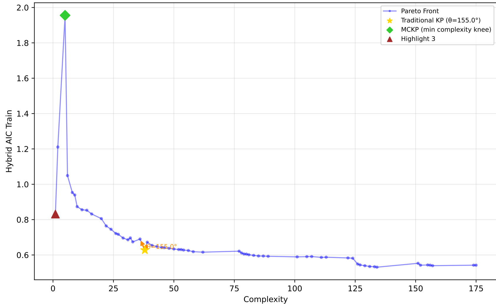
561_cpu - Run 1 - SVP - Hybrid AIC Train \lambda_1=0.90, \lambda_2=0.00, \lambda_3=0.30 | Difficulty: 0.94 | Method: hmr
