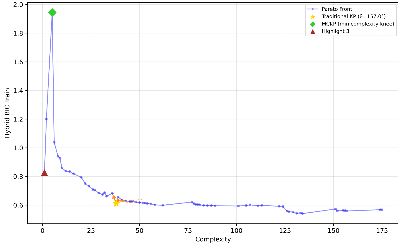
561_cpu - Run 1 - SVP - Hybrid BIC Train \lambda_1=0.90, \lambda_2=0.00, \lambda_3=0.30 | Difficulty: 0.94 | Method: hmr
