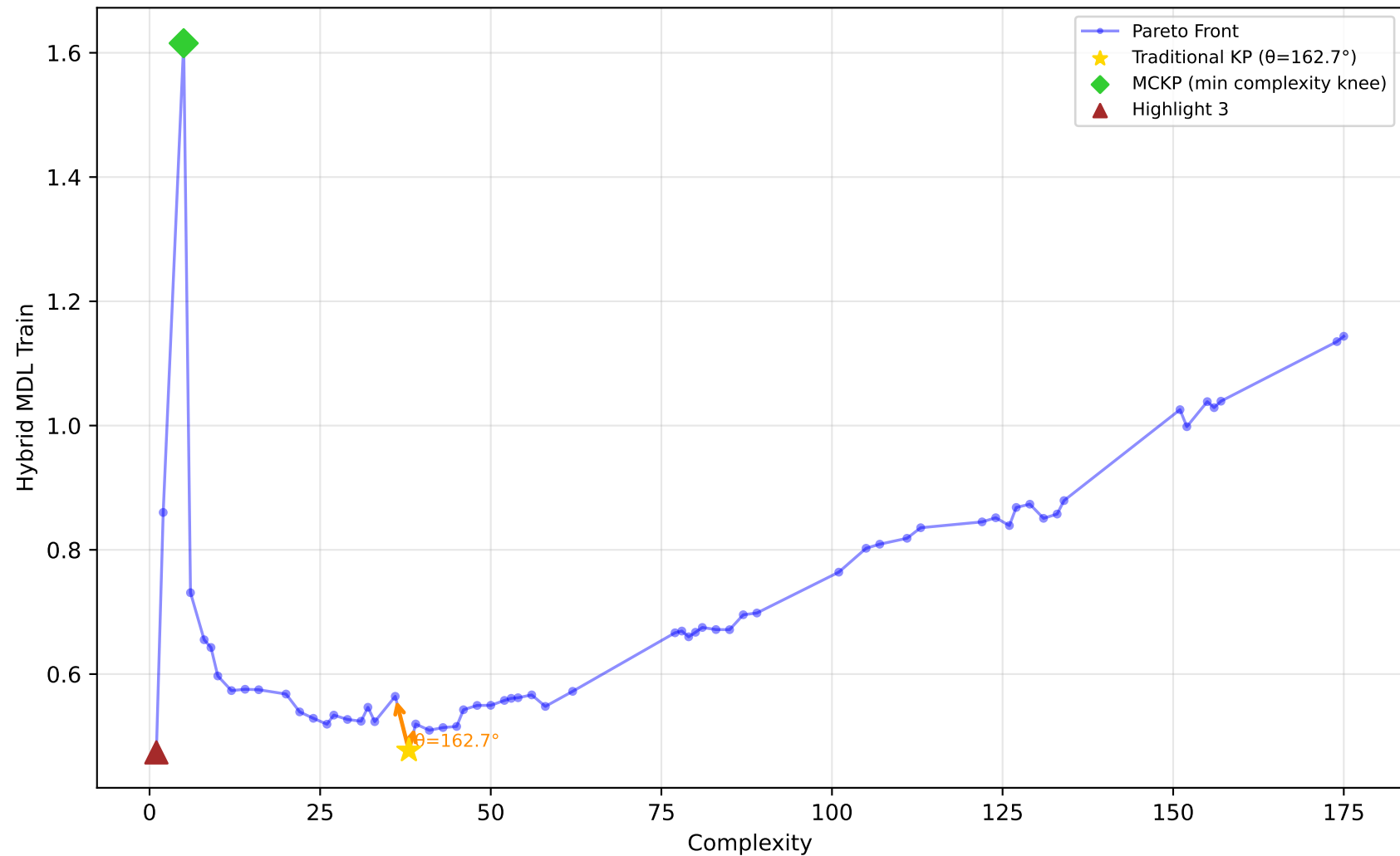
561_cpu - Run 1 - SVP - Hybrid MDL Train \lambda_1=0.90, \lambda_2=0.00, \lambda_3=0.30 | Difficulty: 0.94 | Method: hmr
