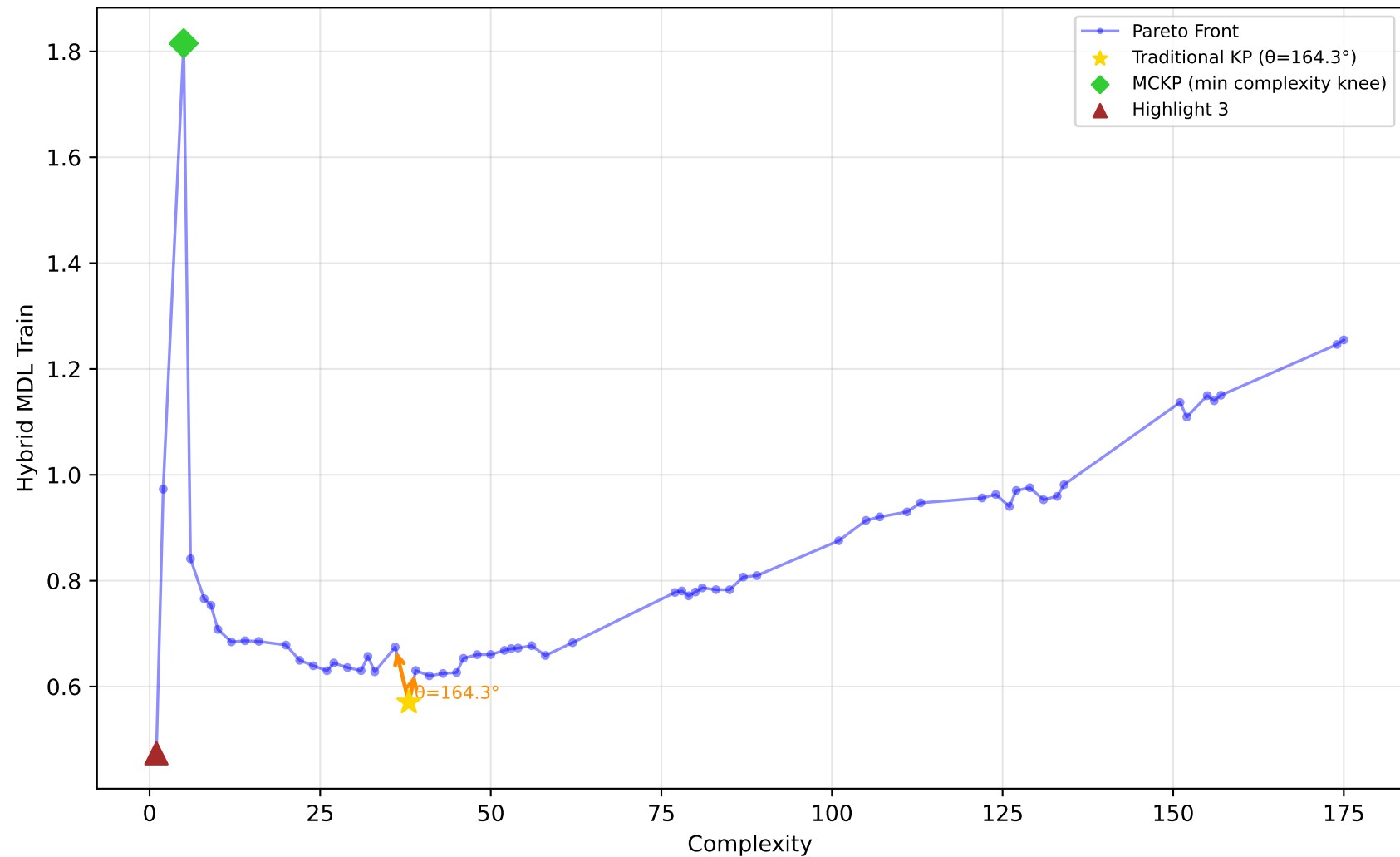
561_cpu - Run 1 - SVP - Hybrid MDL Train \lambda_1=1.00, \lambda_2=0.00, \lambda_3=0.40 | Difficulty: 0.94 | Method: hmr
