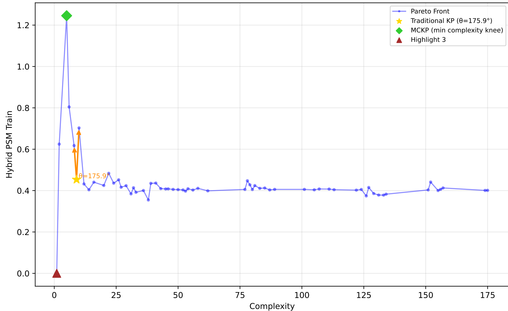
561_cpu - Run 1 - SVP - Hybrid PSM Train \lambda_1=0.90, \lambda_2=0.00, \lambda_3=0.30 | Difficulty: 0.94 | Method: hmr
