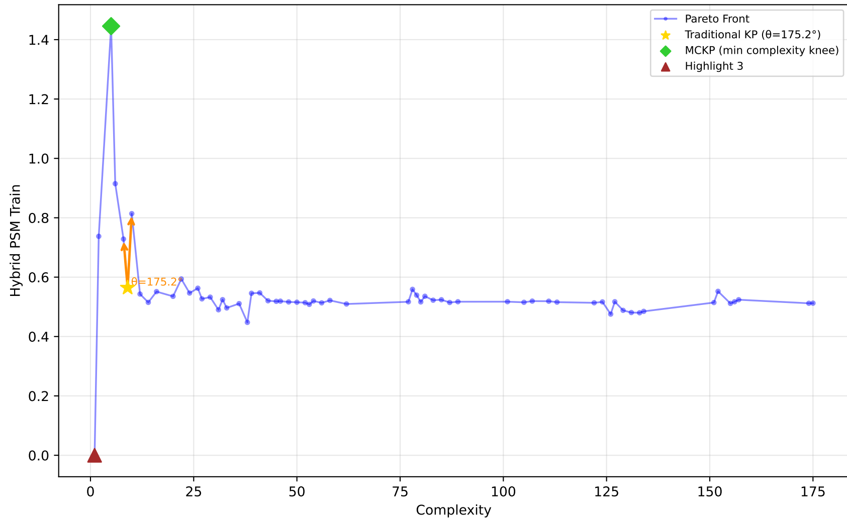
561_cpu - Run 1 - SVP - Hybrid PSM Train \lambda_1=1.00, \lambda_2=0.00, \lambda_3=0.40 | Difficulty: 0.94 | Method: hmr
