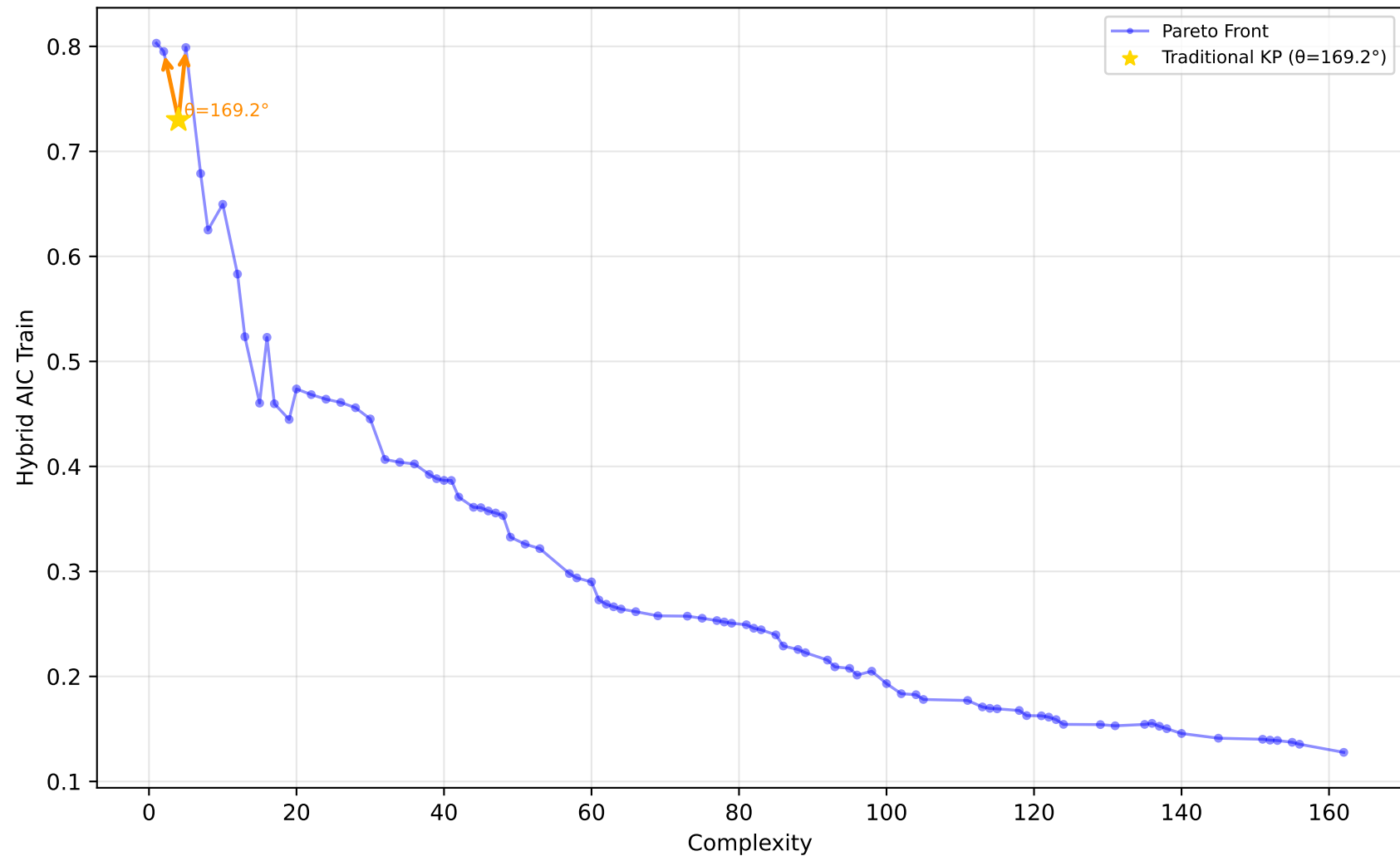
561_cpu - Run 20 - MVP - Hybrid AIC Train \lambda_1=0.70, \lambda_2=0.00, \lambda_3=0.10 | Difficulty: 1.00 | Method: hmr
